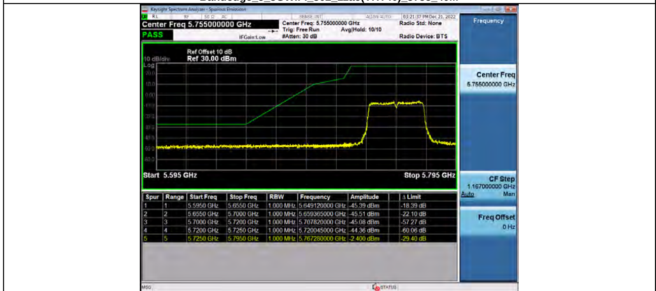
Bandedge_5_8WiFi_802_11ac(VHT40)_5755_40M
