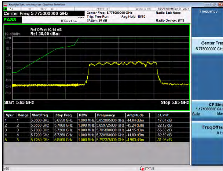
Bandedge 5 8WiFi 802_11ac(VHT80) 5775 80M up
