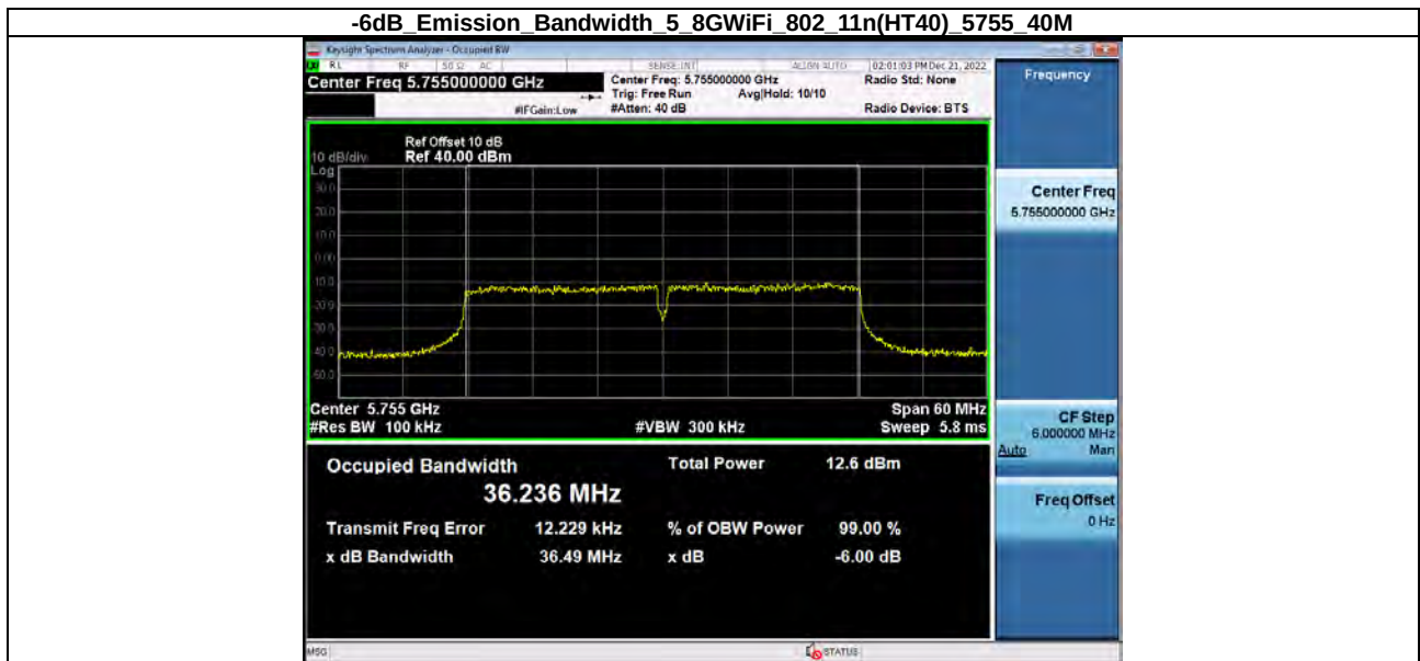
-6dB Emission Bandwidth 5_8WiFi 802_11n(HT40)_5795_40M
