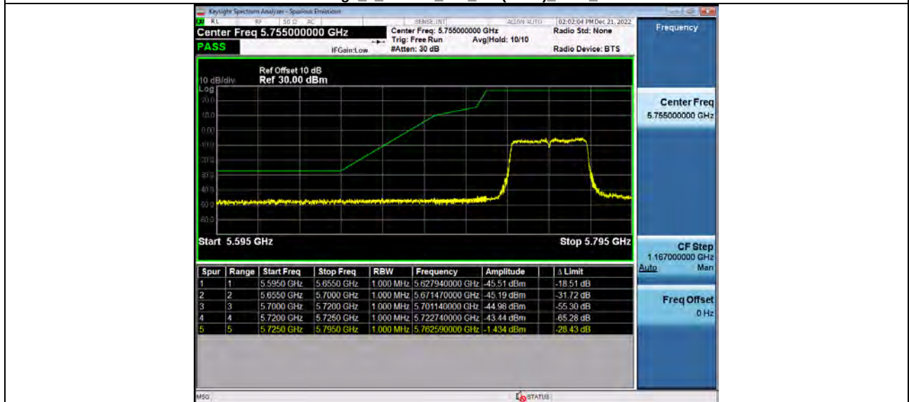
Bandedge_5_8WiFi_802_11n(HT40)_5755_40M
