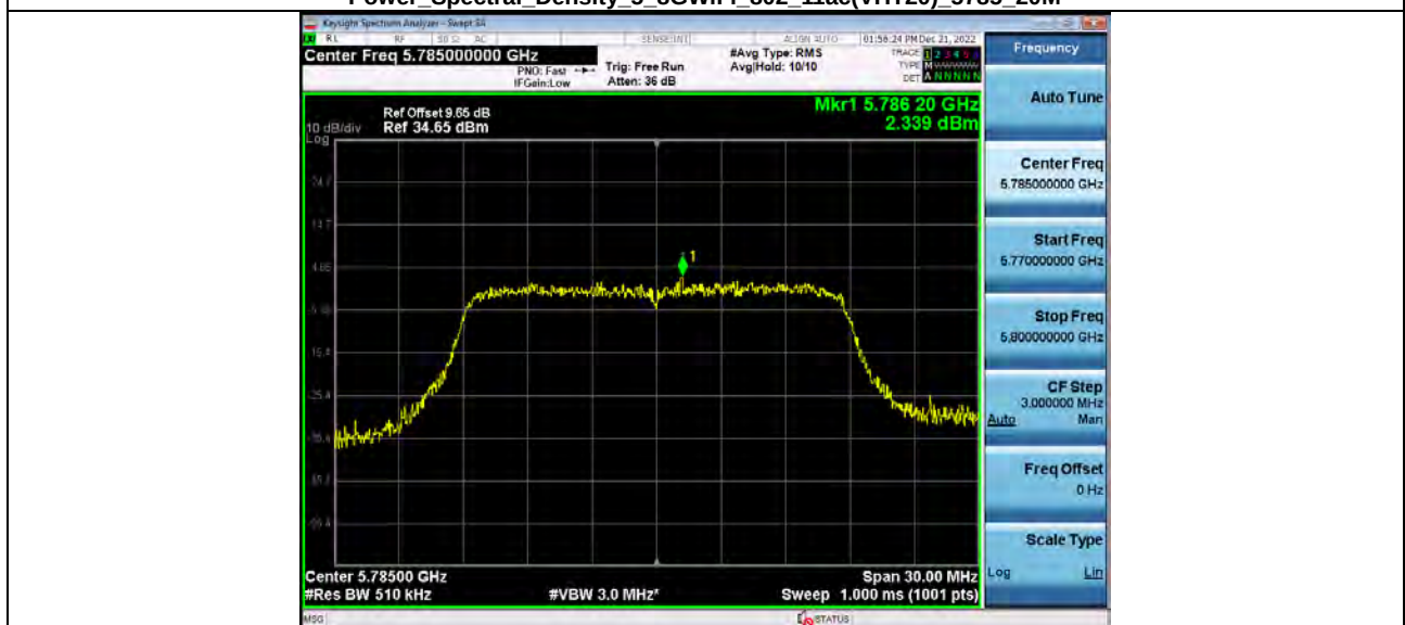
Power Spectral Density 5_8WiFi 802_11ac(VHT20)_5785_20M
