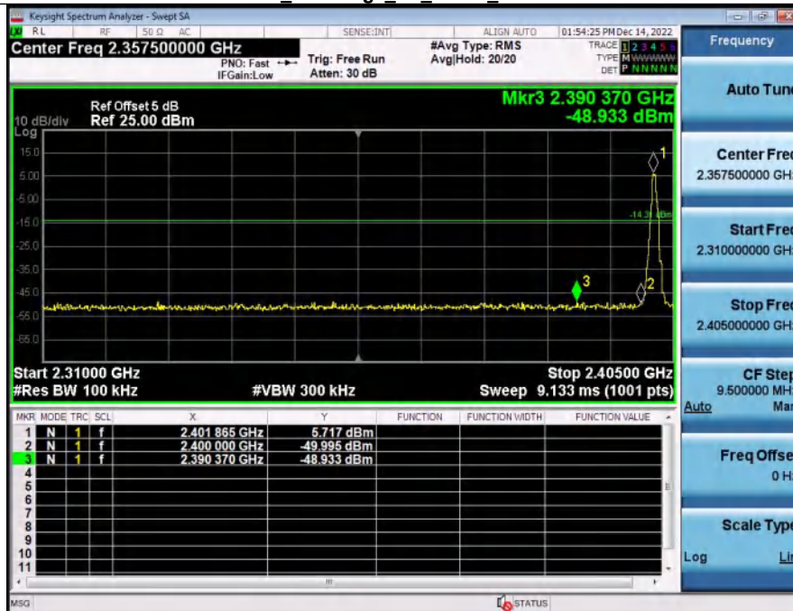
2_Bandedge_BT_1-DH5_2402
