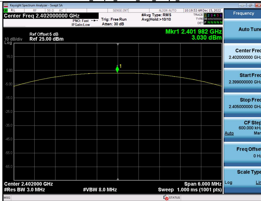
Peak_Output_Power_BLE_1Mbps_2402
