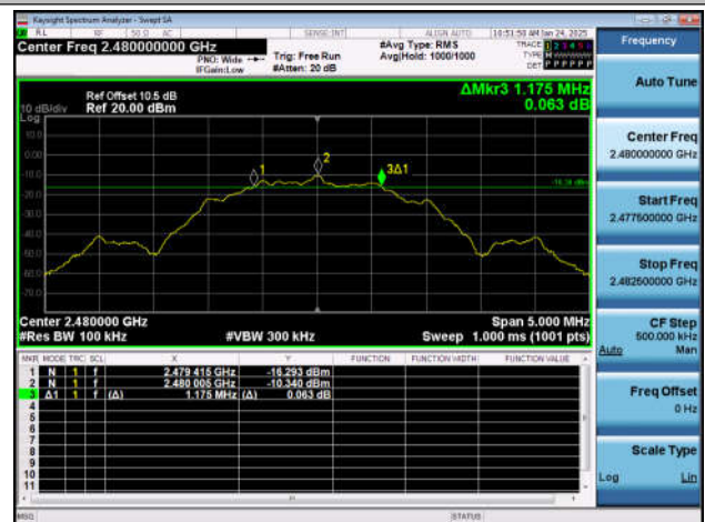
BLE_2M-Ant1-2480-PASS
