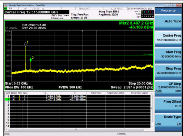
BLE_2M-Ant1-2480-30~25000-PASS
