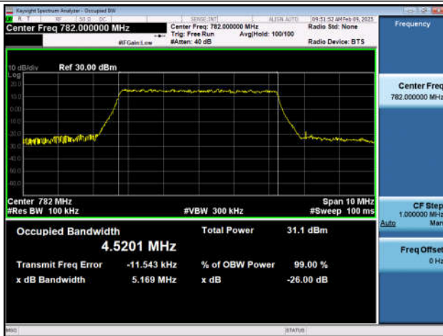
Band13-5MHz-QPSK-23230-25RB#0-PASS
