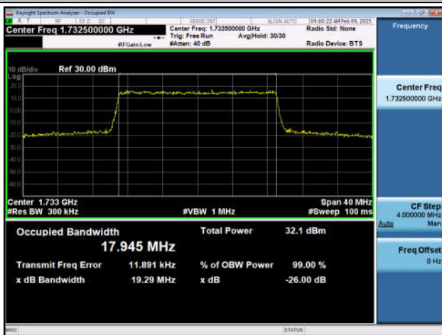
Band4-20MHz-QPSK-20175-100RB#0-PASS
