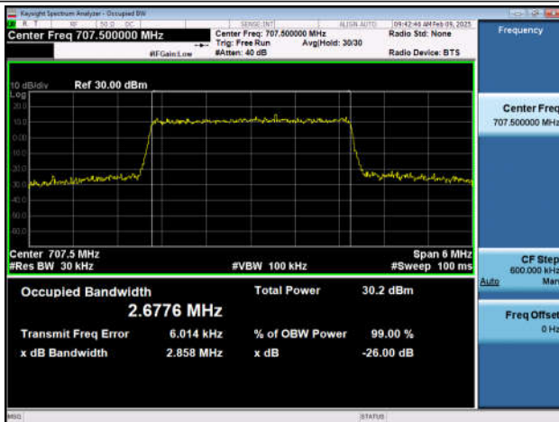
Band12-5MHz-QPSK-23095-25RB#0-PASS
