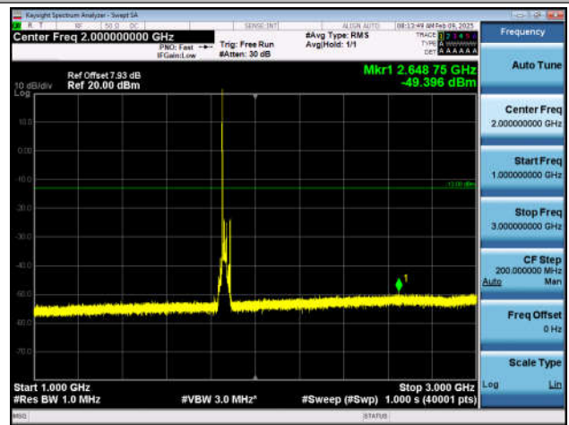
Band2_20MHz_QPSK_18700_1RB#0_1000~3000_1000~3000
