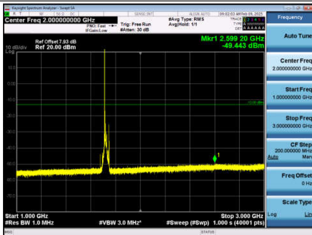
Band4_20MHz_QPSK_20050_1RB#0_1000~3000_1000~3000
