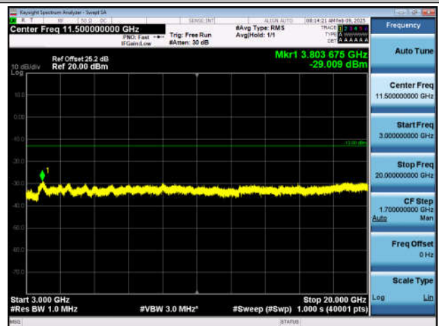
Band2_20MHz_QPSK_18900_1RB#0_3000~20000_3000~20000
