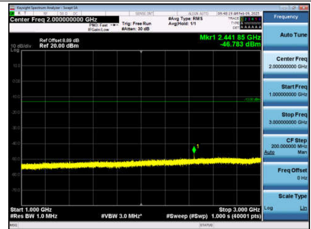
Band12_10MHz_QPSK_23095_1RB#0_1000~3000_1000~3000
