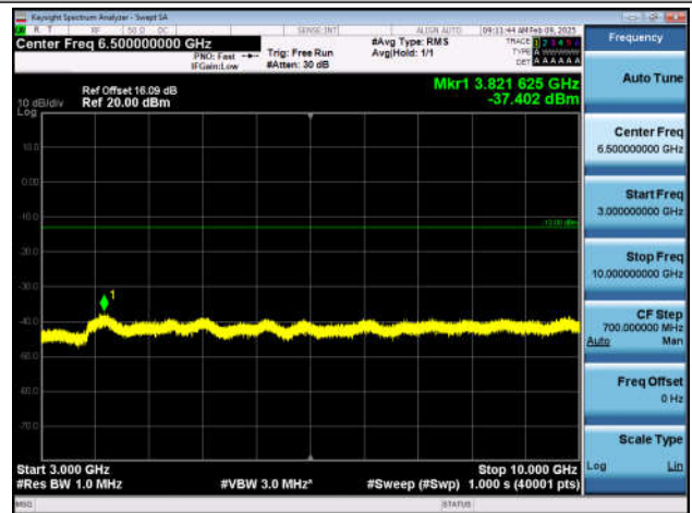
Band5_10MHz_QPSK_20525_1RB#0_3000~10000_3000~10000
