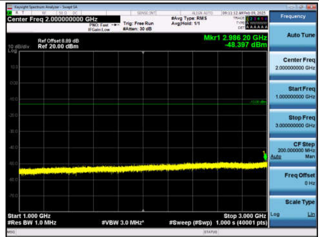
Band5_10MHz_QPSK_20450_1RB#0_1000~3000_1000~3000
