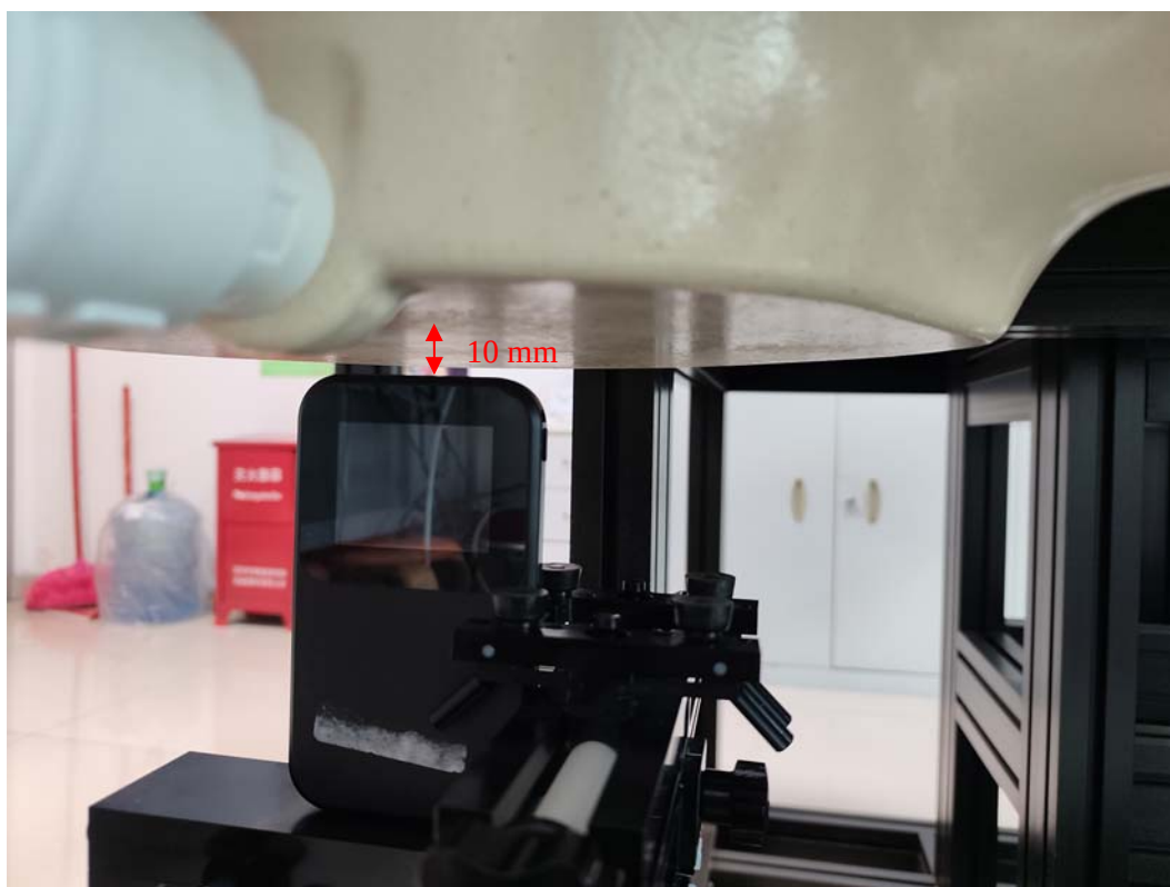
Ant 0 Body Bottom Setup Photo (10 mm)
