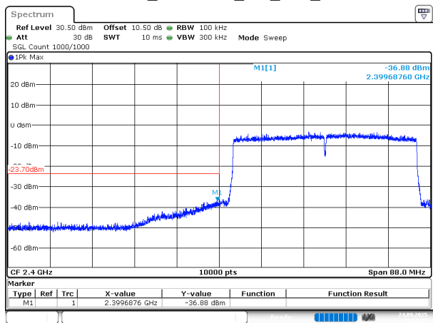
802.11ax40_2422MHz_RU_Full_Chain 0
