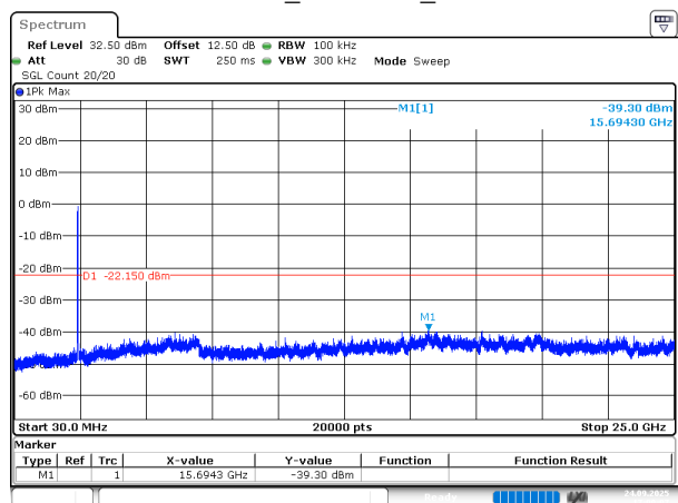
802.11n40_2422MHz_Chain 1
