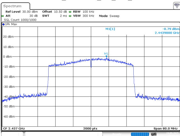
802.11ax40_2437MHz_RU_Full_Chain 1
