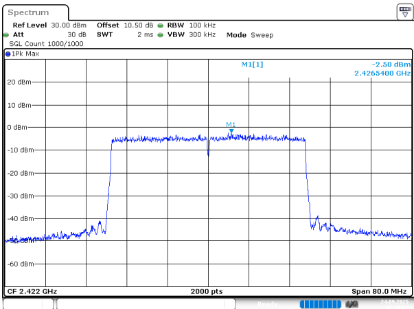
802.11ax40_2422MHz_RU_Full_Chain 1
