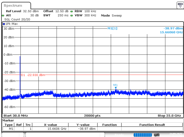
802.11ax40_2452MHz_RU_Full_Chain 0
