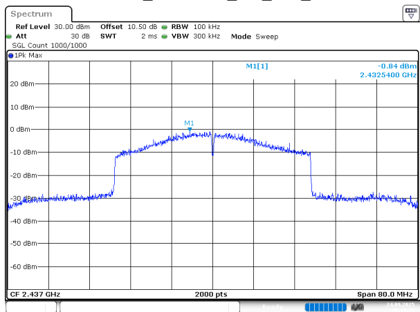
802.11ax40_2437MHz_RU_Full_Chain 0
