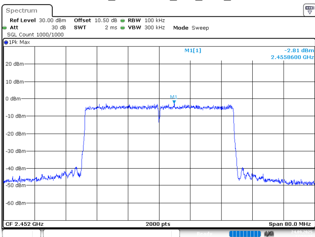
802.11ax40_2452MHz_RU_Full_Chain 1
