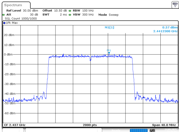
802.11ax20_2437MHz_RU_Full_Chain 1
