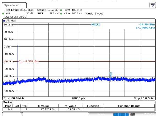
802.11ax20_2462MHz_RU_Full_Chain 1
