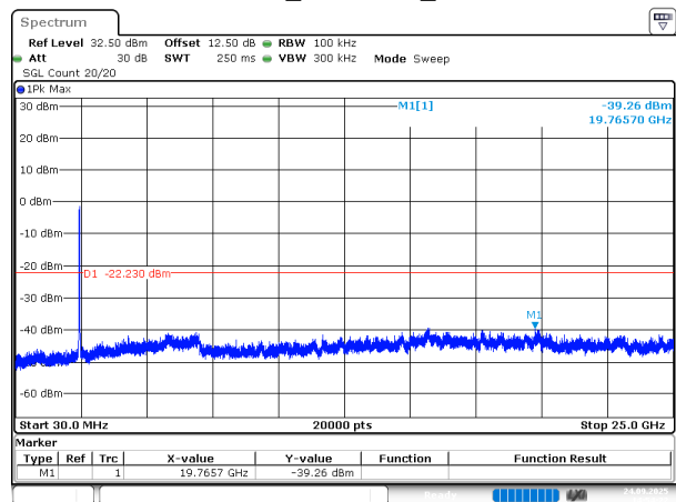
802.11n40_2452MHz_Chain 0
