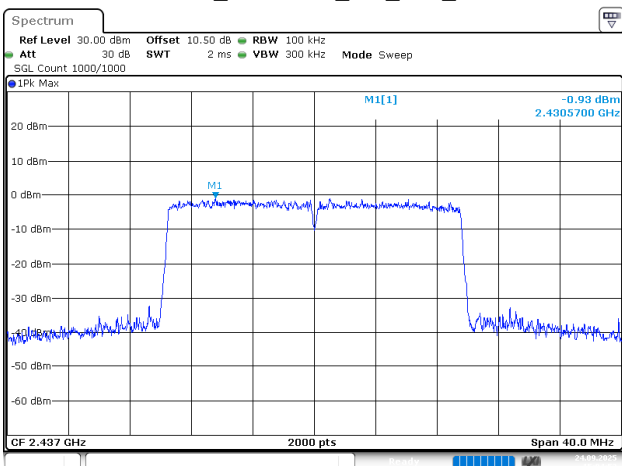
802.11ax20_2437MHz_RU_Full_Chain 0
