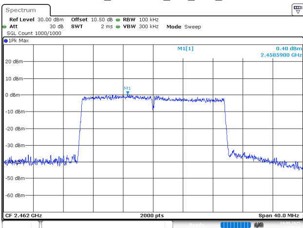
802.11ax20_2462MHz_RU_Full_Chain 0
