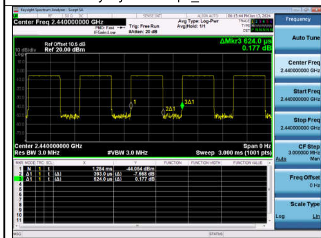
Duty Cycle: 1Mbps_2440MHz
