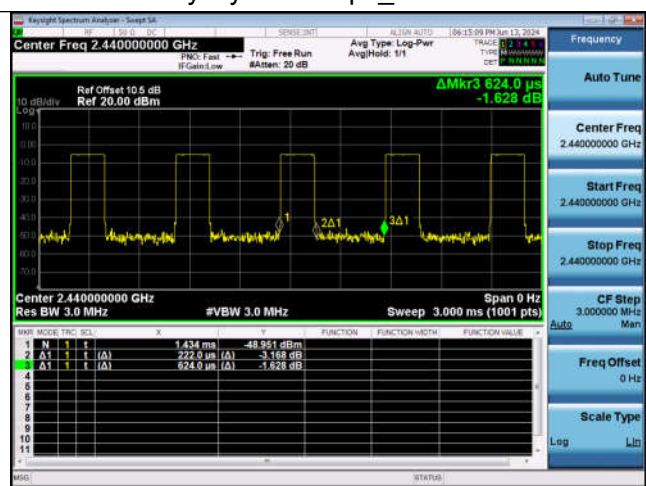
Duty Cycle: 2Mbps_2440MHz
