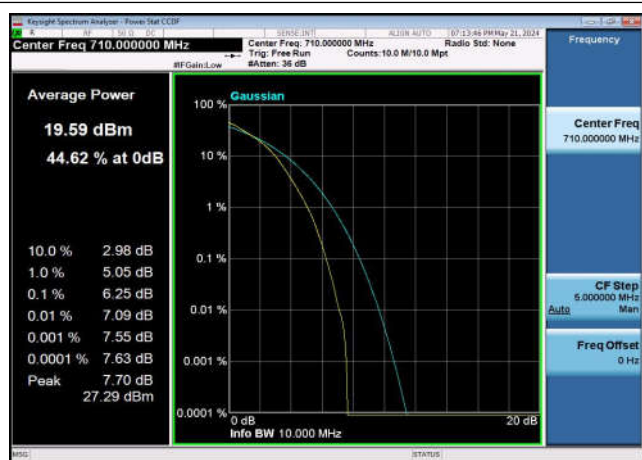
FDD17_MidRange_10MHz_710_fullIRB _Q16
