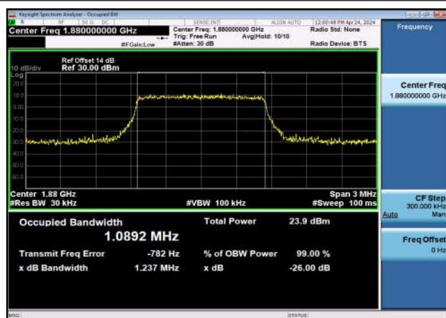
FDD02_MidRange_10_1880_QPSK
