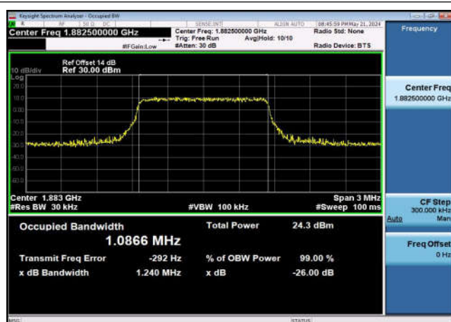
FDD25_MidRange_1.4_1882.5_QPSK
