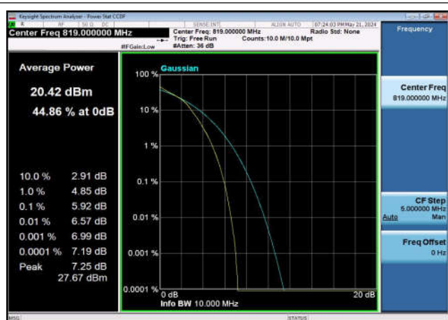
FDD26_Part 90_LowRange_10MHz_819_fullRB_Q16
