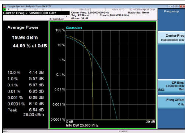
TDD41_MidRange_20MHz_2605_OneRB _high_Q16
