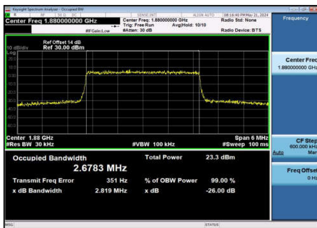
FDD02_MidRange_5_1880_Q16
