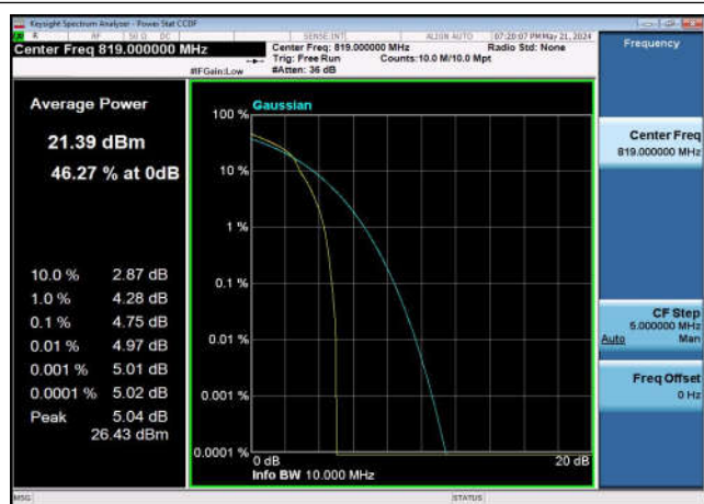
FDD26_Part 90_MidRange_10MHz_819_fullRB_Q16
