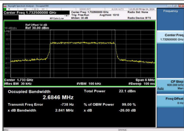
FDD04_MidRange_5_1732.5_QPSK
