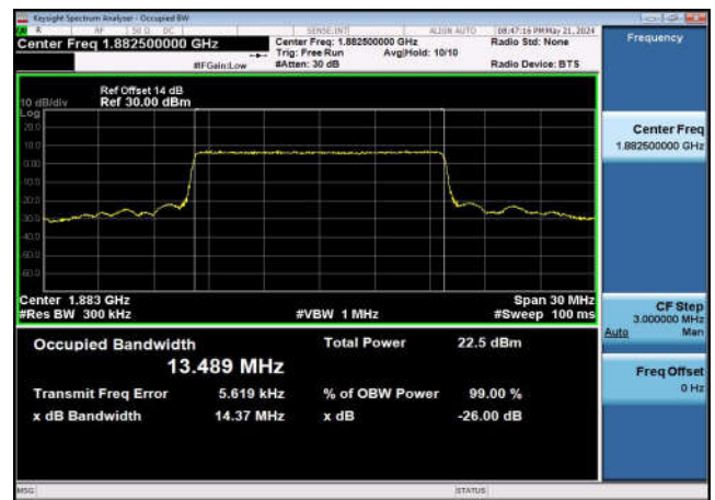
FDD25_MidRange_20_1882.5_QPSK
