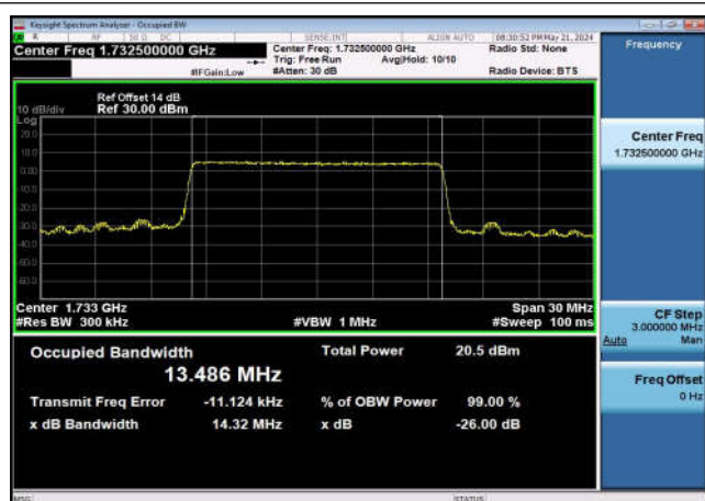
FDD04_MidRange_15_1732.5_QPSK
