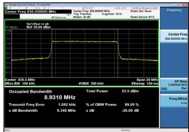
FDD26_Part 22_MidRange_15_836.5_QPSK
