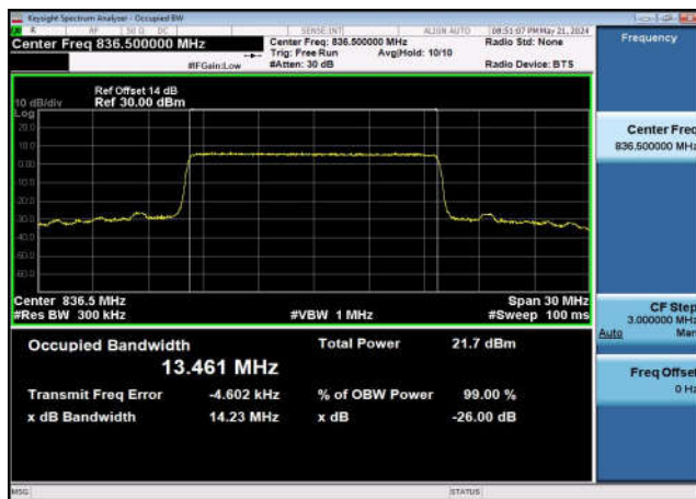
FDD26_Part 22_MidRange_3_836.5_Q16
