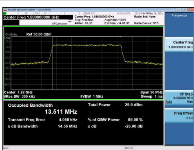
FDD02_MidRange_15_1880_Q16
