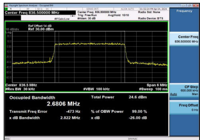
FDD26_Part 22_MidRange_3_836.5_QPSK
