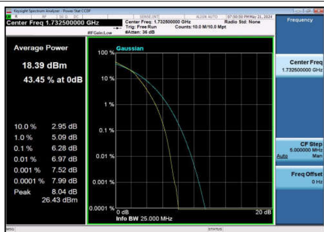
FDD04_MidRange_20MHz_1732.5_fullIRB _Q16
