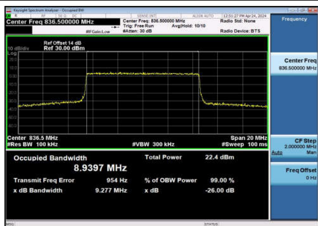
FDD05_MidRange_3_836.5_Q16
