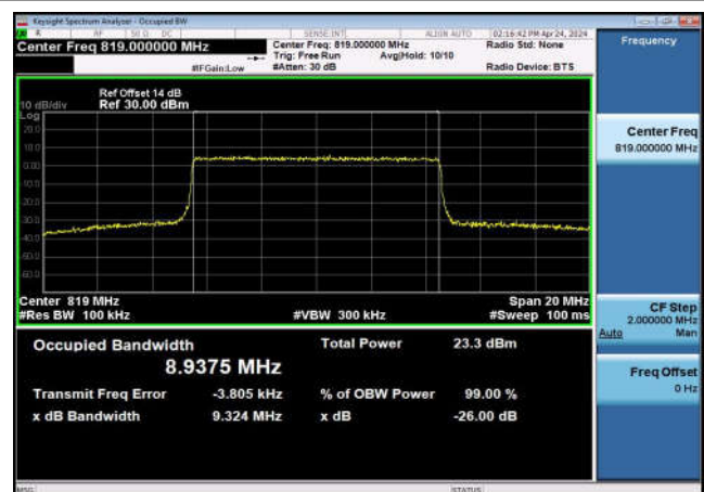
FDD26_Part 90_MidRange_10_819_QPSK
