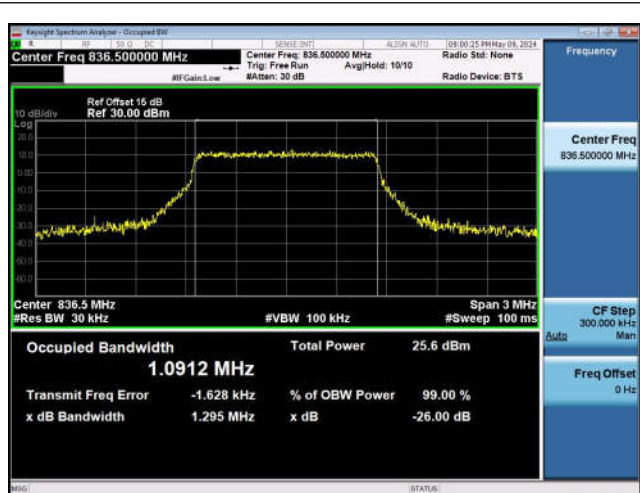
FDD26_Part 22_MidRange_1.4_836.5_Q16
