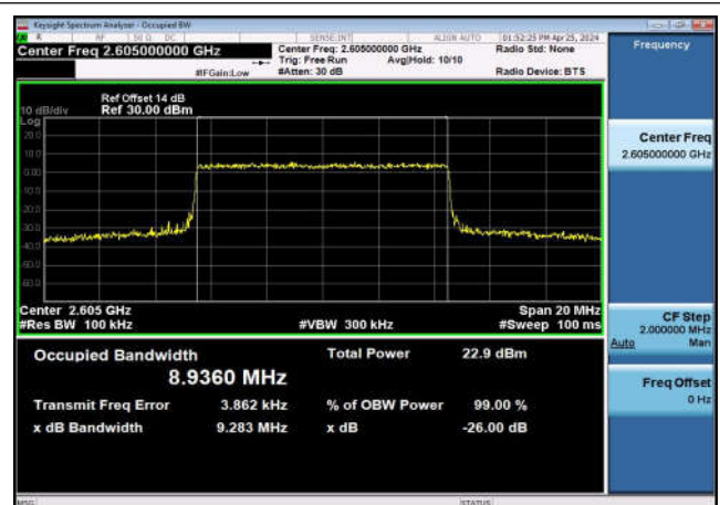
TDD41_MidRange_10_2605_QPSK
