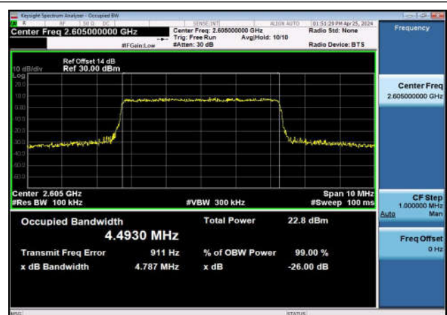
TDD41_MidRange_5_2605_QPSK
