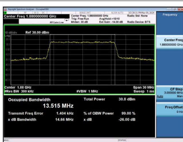
FDD02_MidRange_15_1880_QPSK
