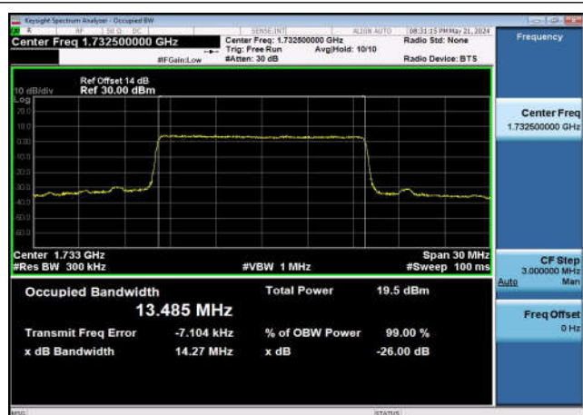
FDD04_MidRange_15_1732.5_Q16
