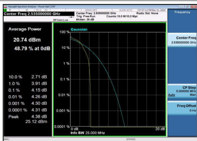
FDD07_MidRange_20MHz_2535_fullIRB _Q16
