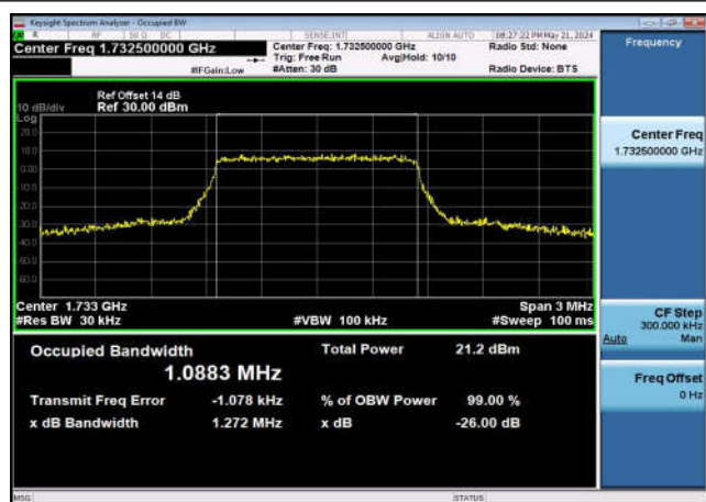
FDD04_MidRange_10_1732.5_Q16
