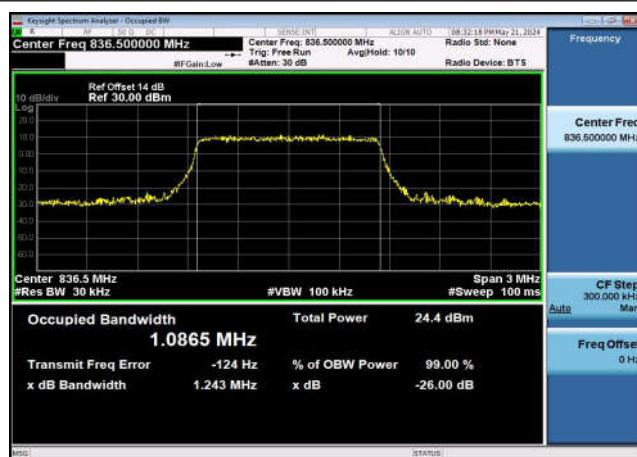
FDD05_MidRange_10_836.5_QPSK
