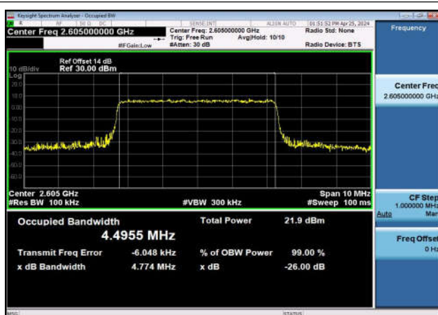
TDD41_MidRange_5_2605_Q16
