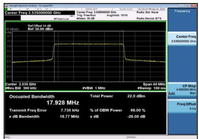
FDD07_MidRange_5_2535_QPSK
