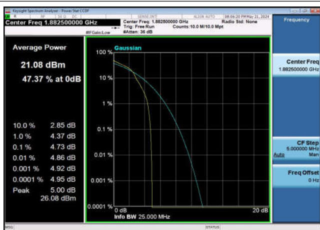
FDD25_MidRange_20MHz_1882.5_OneRB _high_Q16
