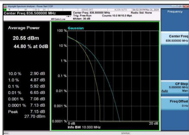
FDD05_MidRange_10MHz_836.5_fullIRB _Q16
