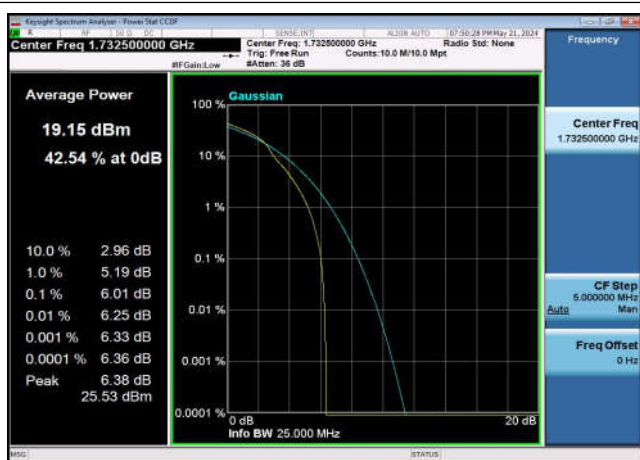
FDD04_MidRange_20MHz_1732.5_OneRB _high_Q16
