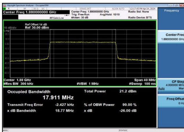
FDD02_MidRange_3_1880_Q16
