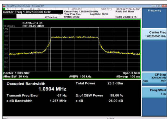
FDD25_MidRange_1.4_1882.5_Q16
