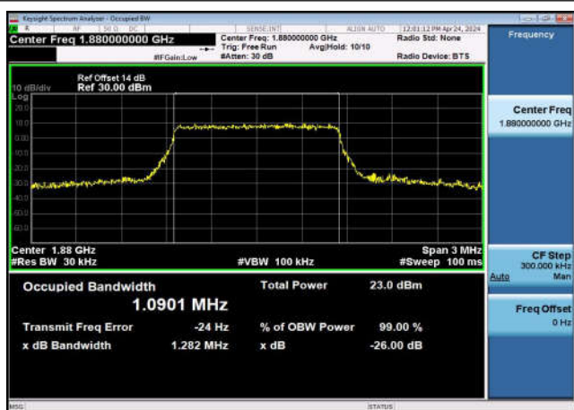
FDD02_MidRange_10_1880_Q16
