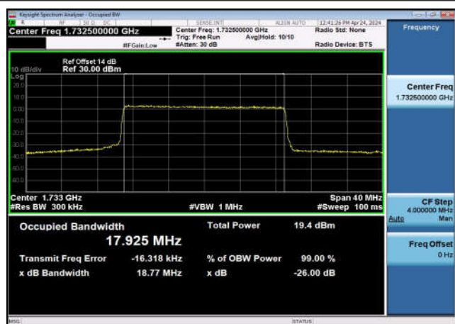
FDD04_MidRange_3_1732.5_Q16
