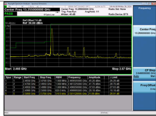
20MHz-10MHz_QPSK@QPSK-QPSK@QPSK_20850-209 94_1RB#0@100RB#0-0RB#0@50RB#0
