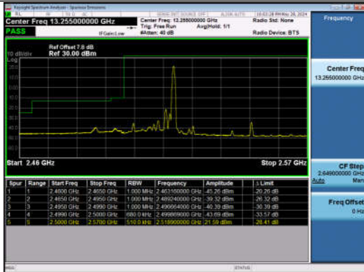
20MHz-15MHz_QPSK@QPSK-QPSK@QPSK_20850-21021 1_1RB#99@100RB#0-0RB#0@75RB#0
