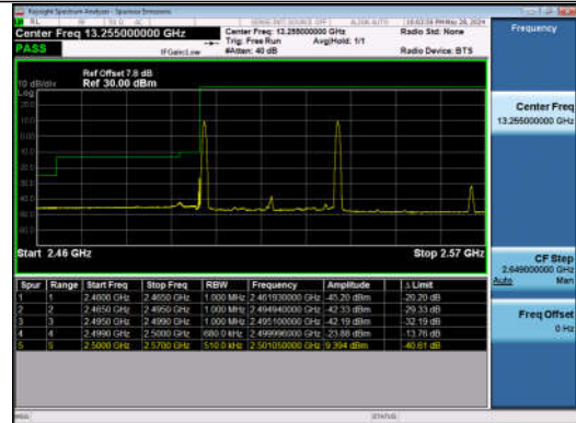
20MHz-15MHz_QPSK@QPSK-QPSK@QPSK_20850-21021 21_1RB#0@100RB#0-1RB#74@75RB#0
