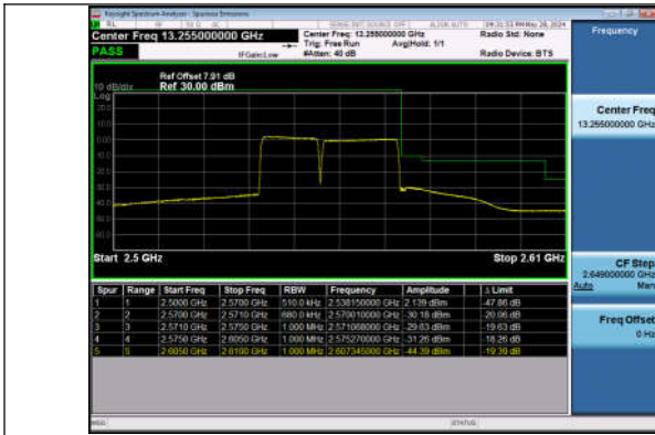
15MHz-20MHz_QPSK@QPSK-QPSK@QPSK_21179-2135 0_75RB#0@75RB#0-100RB#0@100RB#0
