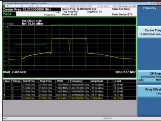
15MHz-15MHz_QPSK@QPSK-QPSK@QPSK_20825-2097 5_75RB#0@75RB#0-75RB#0@75RB#0
