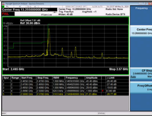
15MHz-15MHz_QPSK@QPSK-QPSK@QPSK_20825-20975_975_1RB#0@75RB#0-0RB#0@75RB#0
