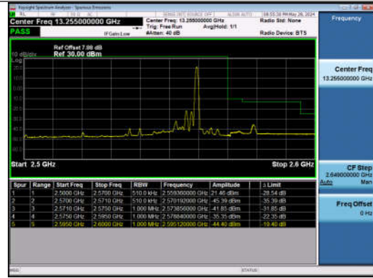
15MHz-10MHz_QPSK@QPSK-QPSK@QPSK_21277-21397_1RB#74@75RB#0-0RB#0@50RB#0
