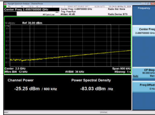
15MHz-15MHz_QPSK@QPSK-QPSK@QPSK_20825-20975_1RB#0@75RB#0-0RB#0@75RB#0_Final1
