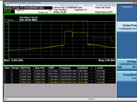
10MHz-20MHz_QPSK@QPSK-QPSK@QPSK_40996-41140_50RB#0@50RB#0-100RB#0@100RB#0
