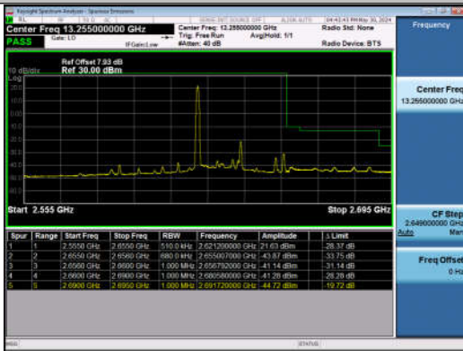
20MHz-15MHz_QPSK@QPSK-QPSK@QPSK_40991-41162_1RB#0@100RB#0-0RB#0@75RB#0
