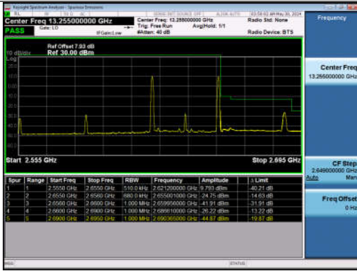
15MHz-20MHz_QPSK@QPSK-QPSK@QPSK_40969-41140_1RB#0@75RB#0-1RB#99@100RB#0
