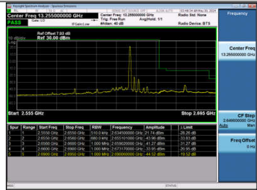
15MHz-20MHz_QPSK@QPSK-QPSK@QPSK_40969-41140_1RB#74@75RB#0-0RB#0@100RB#0
