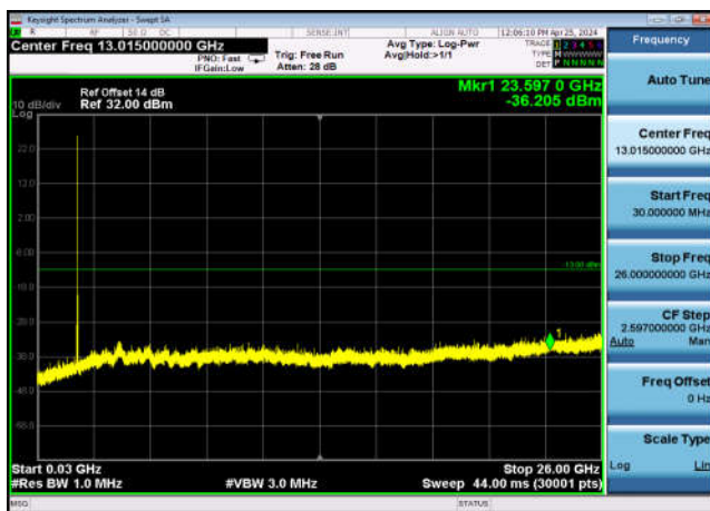
FDD04_LowRange_20MHz_30MHz~26GHz
