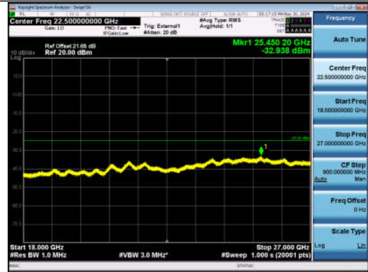
41-41-20MHz-20MHz-QPSK-QPSK-40942-41140-1RB#0-0 RB#0-18000~27000MHz-PASS
