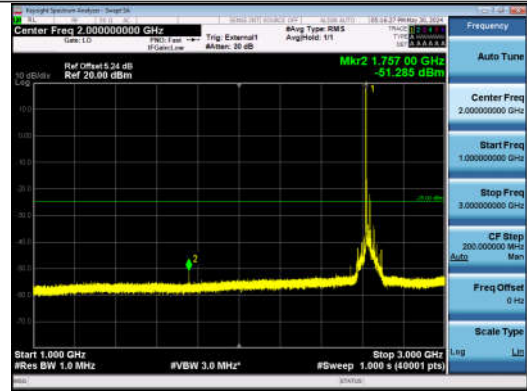
41-41-20MHz-20MHz-QPSK-QPSK-40942-41140-1RB#0-0 RB#0-1000~3000MHz-PASS
