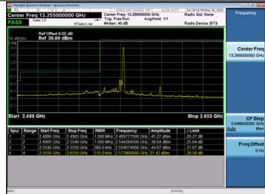
20MHz-15MHz_QPSK@QPSK-QPSK@QPSK_40340-40511_1RB#99@100RB#0-0RB#0@75RB#0
