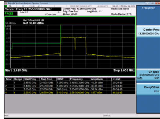
20MHz-15MHz_QPSK@QPSK-QPSK@QPSK_40340-40511_100RB#0@100RB#0-75RB#0@75RB#0
