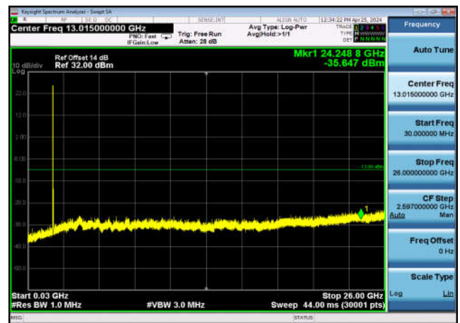
FDD26_Part 22_HighRange_15MHz_30MHz~26GHz
