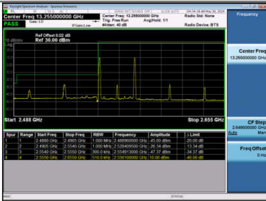
20MHz-10MHz_QPSK@QPSK-QPSK@QPSK_40340-40484_1RB#0@100RB#0-1RB#49@50RB#0
