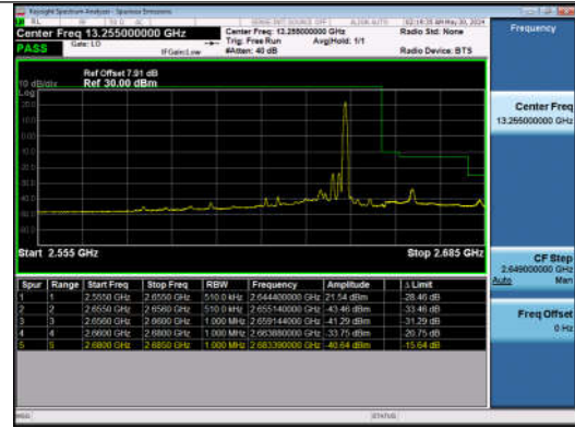
15MHz-10MHz_QPSK@QPSK-QPSK@QPSK_41067-41187_1RB#74@75RB#0-0RB#0@50RB#0
