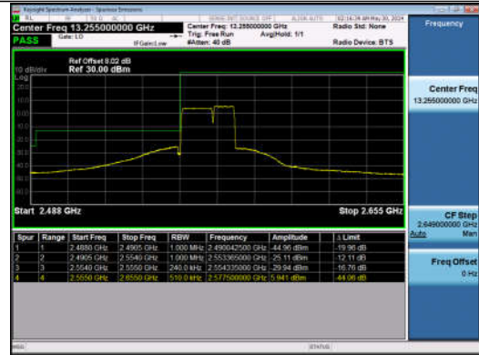
15MHz-10MHz_QPSK@QPSK-QPSK@QPSK_40315-40435_75RB#0@75RB#0-50RB#0@50RB#0
