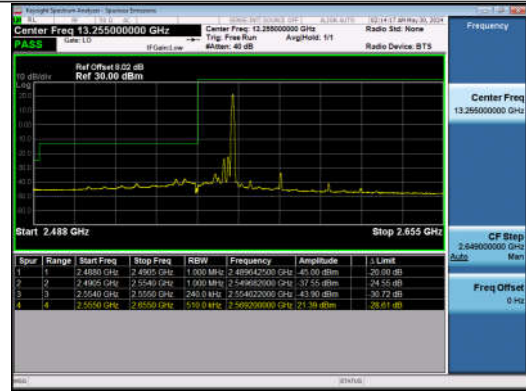
15MHz-10MHz_QPSK@QPSK-QPSK@QPSK_40315-40435_1RB#74@75RB#0-0RB#0@50RB#0
