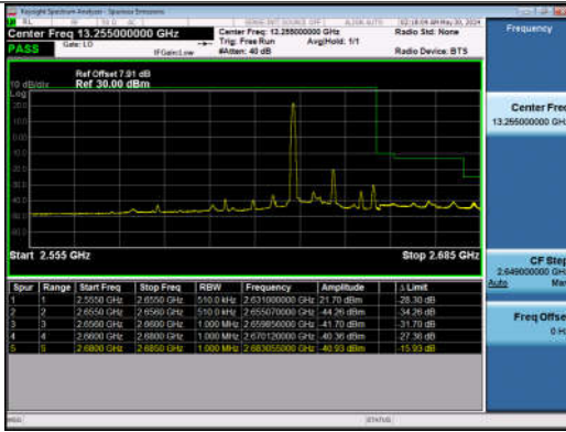
15MHz-10MHz_QPSK@QPSK-QPSK@QPSK_41067-41187_1RB#0@75RB#0-0RB#0@50RB#0
