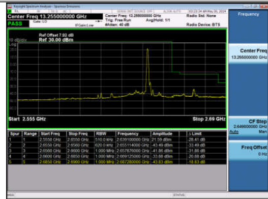
15MHz-15MHz_QPSK@QPSK-QPSK@QPSK_41015-41165_1RB#74@75RB#0-0RB#0@75RB#0
