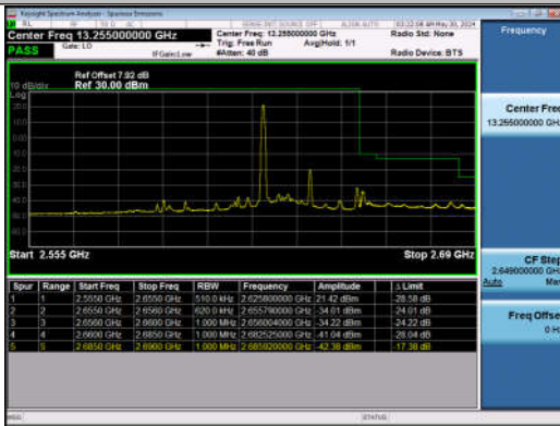
15MHz-15MHz_QPSK@QPSK-QPSK@QPSK_41015-41165_165_1RB#0@75RB#0-0RB#0@75RB#0
