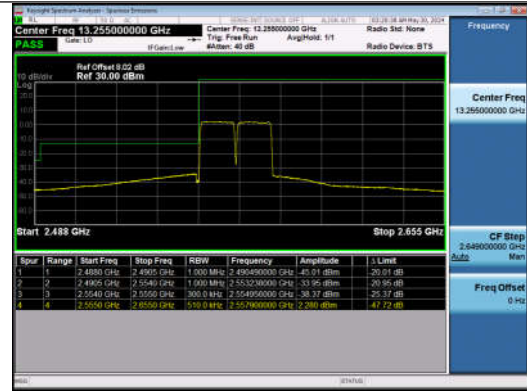
15MHz-15MHz_QPSK@QPSK-QPSK@QPSK_40315-40465_75RB#0@75RB#0-75RB#0@75RB#0
