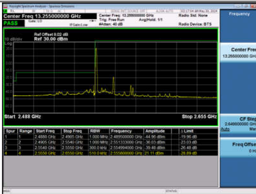
15MHz-15MHz_QPSK@QPSK-QPSK@QPSK_40315-40465_465_1RB#0@75RB#0-0RB#0@75RB#0
