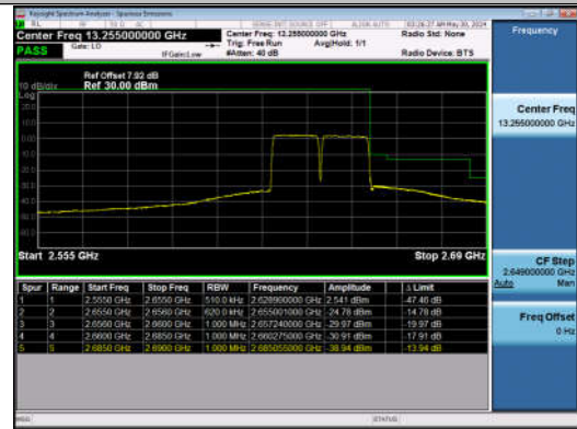
15MHz-15MHz_QPSK@QPSK-QPSK@QPSK_41015-41165_75RB#0@75RB#0-75RB#0@75RB#0
