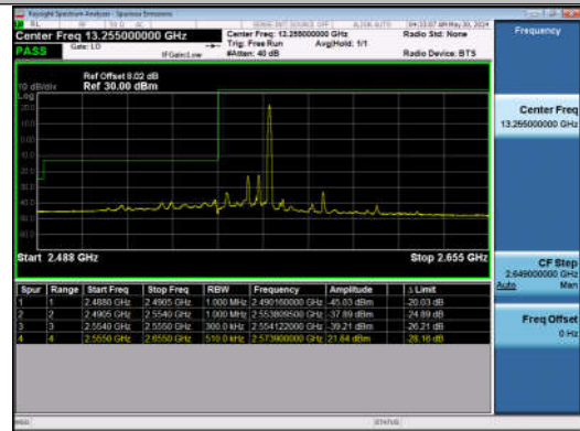
20MHz-10MHz_QPSK@QPSK-QPSK@QPSK_40340-40484_1RB#99@100RB#0-0RB#0@50RB#0
