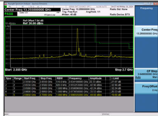
20MHz-20MHz_QPSK@QPSK-QPSK@QPSK_40942-41140_1RB#99@100RB#0-0RB#0@100RB#0
