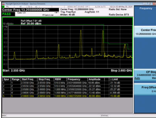
15MHz-10MHz_QPSK@QPSK-QPSK@QPSK_41067-41187_1RB#0@75RB#0-1RB#49@50RB#0
