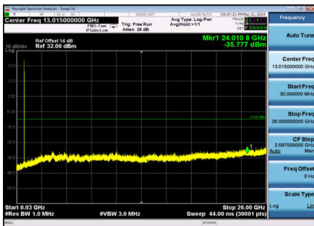
FDD07_LowRange_20MHz_30MHz~26GHz
