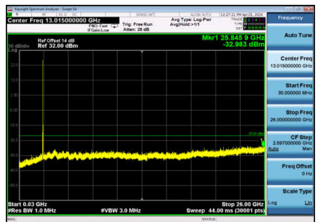
FDD07_MidRange_20MHz_30MHz~26GHz
