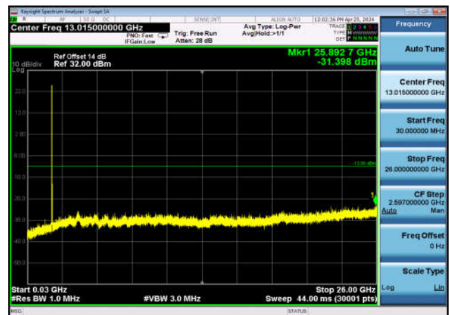
FDD04_HighRange_20MHz_30MHz~26GHz
