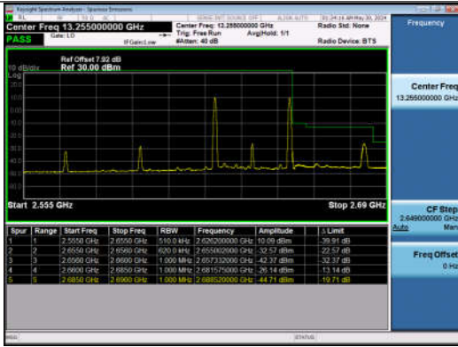
10MHz-20MHz_QPSK@QPSK-QPSK@QPSK_40996-41140_1RB#0@50RB#0-1RB#99@100RB#0
