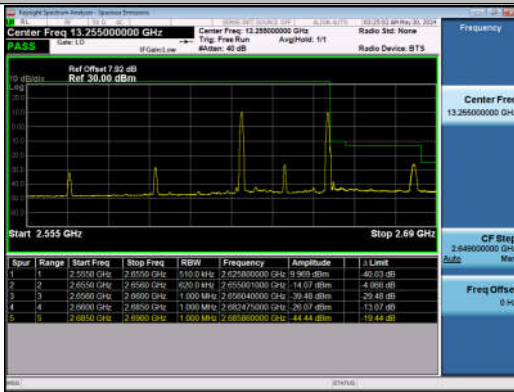
15MHz-15MHz_QPSK@QPSK-QPSK@QPSK_41015-41165_165_1RB#0@75RB#0-1RB#74@75RB#0
