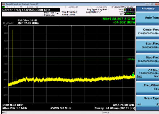
FDD05_MidRange_10MHz_30MHz~26GHz
