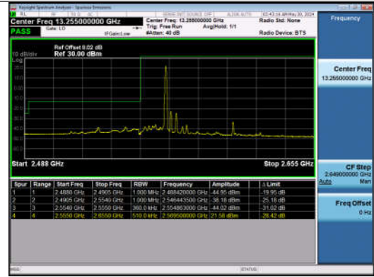
15MHz-20MHz_QPSK@QPSK-QPSK@QPSK_40318-40489_1RB#74@75RB#0-0RB#0@100RB#0
