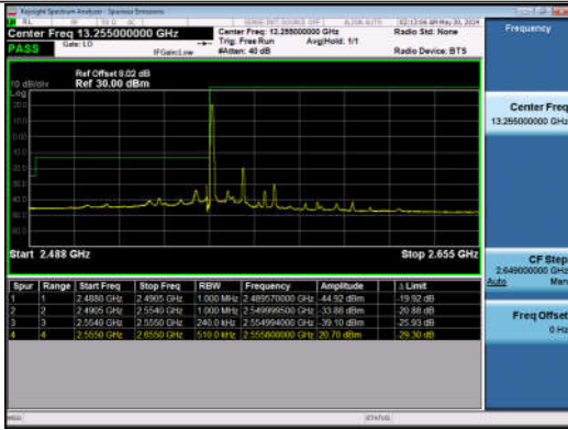
15MHz-10MHz_QPSK@QPSK-QPSK@QPSK_40315-40435_435_1RB#0@75RB#0-0RB#0@50RB#0
