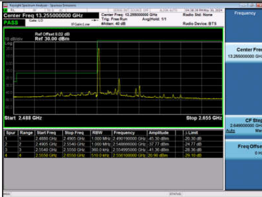
20MHz-15MHz_QPSK@QPSK-QPSK@QPSK_40340-40511_511_1RB#0@100RB#0-0RB#0@75RB#0
