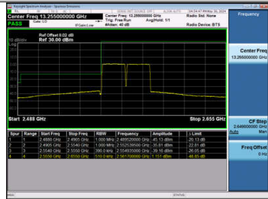
20MHz-20MHz_QPSK@QPSK-QPSK@QPSK_40340-40538_100RB#0@100RB#0-100RB#0@100RB#0
