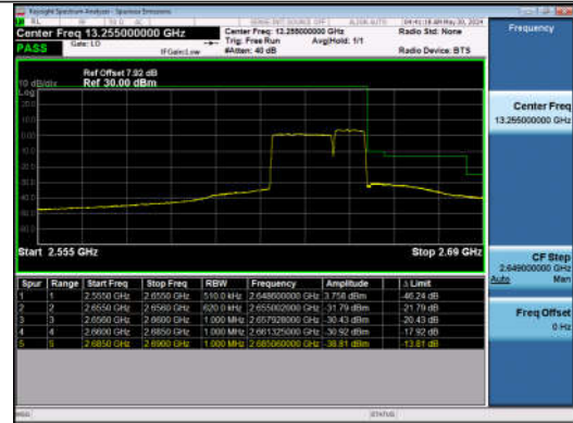
20MHz-10MHz_QPSK@QPSK-QPSK@QPSK_41041-41185_100RB#0@100RB#0-50RB#0@50RB#0
