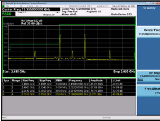
20MHz-15MHz_QPSK@QPSK-QPSK@QPSK_40340-40511_1RB#0@100RB#0-1RB#74@75RB#0
