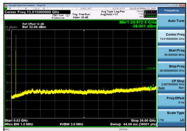
FDD26_Part 22_MidRange_15MHz_30MHz~26GHz
