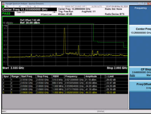
15MHz-20MHz_QPSK@QPSK-QPSK@QPSK_40969-41140_140_1RB#0@75RB#0-0RB#0@100RB#0
