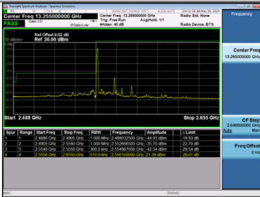
20MHz-10MHz_QPSK@QPSK-QPSK@QPSK_40340-40484_1RB#0@100RB#0-0RB#0@50RB#0
