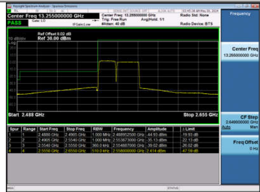
15MHz-20MHz_QPSK@QPSK-QPSK@QPSK_40318-40489_75RB#0@75RB#0-100RB#0@100RB#0
