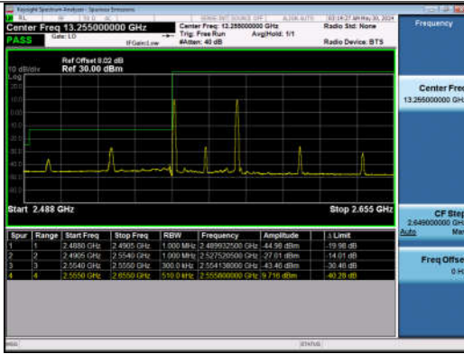
15MHz-15MHz_QPSK@QPSK-QPSK@QPSK_40315-40465_1RB#0@75RB#0-1RB#74@75RB#0
