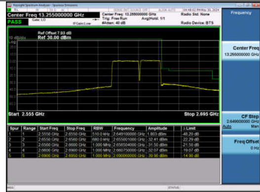
20MHz-15MHz_QPSK@QPSK-QPSK@QPSK_40991-41162_100RB#0@100RB#0-75RB#0@75RB#0
