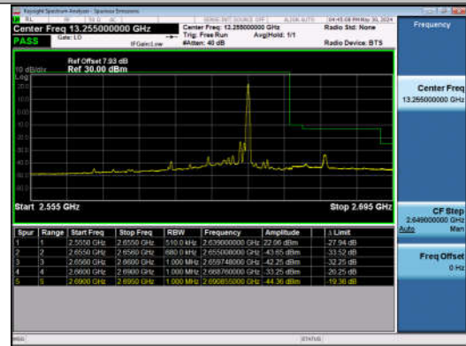
20MHz-15MHz_QPSK@QPSK-QPSK@QPSK_40991-41162_1RB#99@100RB#0-0RB#0@75RB#0
