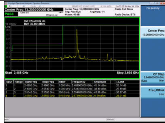
20MHz-20MHz_QPSK@QPSK-QPSK@QPSK_40340-40538_1RB#99@100RB#0-0RB#0@100RB#0
