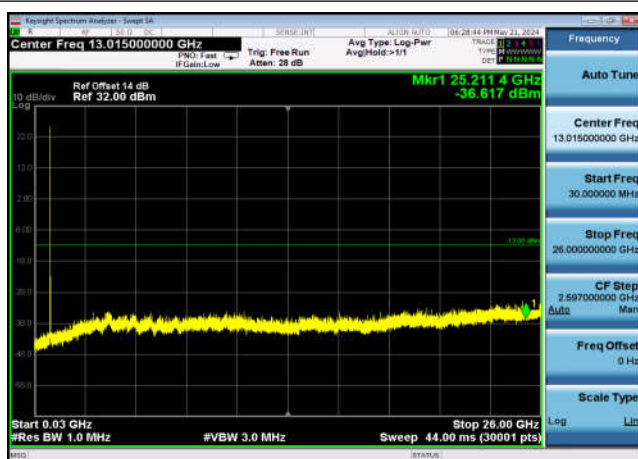
FDD26_Part 22_LowRange_15MHz_30MHz~26GHz
