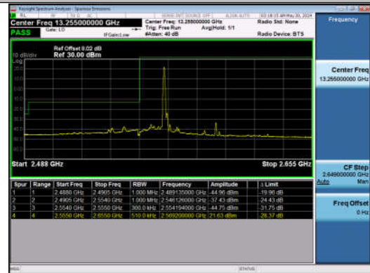
15MHz-15MHz_QPSK@QPSK-QPSK@QPSK_40315-40465_1RB#74@75RB#0-0RB#0@75RB#0
