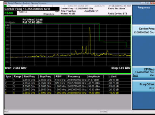
20MHz-10MHz_QPSK@QPSK-QPSK@QPSK_41041-41185_1RB#99@100RB#0-0RB#0@50RB#0
