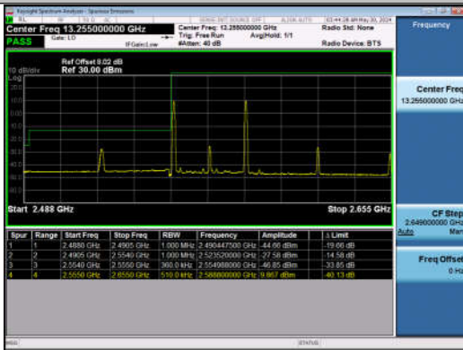
15MHz-20MHz_QPSK@QPSK-QPSK@QPSK_40318-40489_1RB#0@75RB#0-1RB#99@100RB#0
