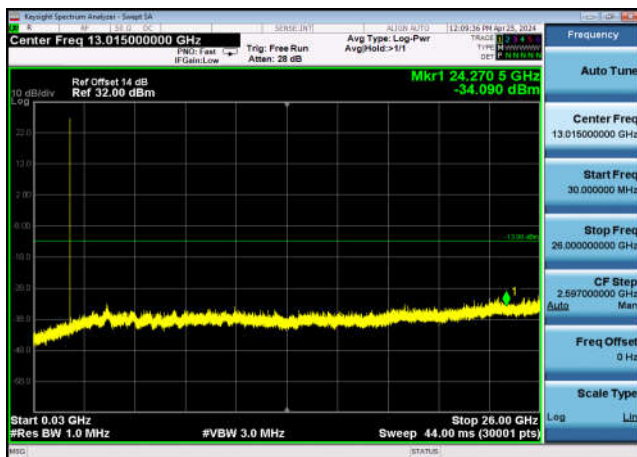
FDD02_MidRange_20MHz_30MHz~26GHz
