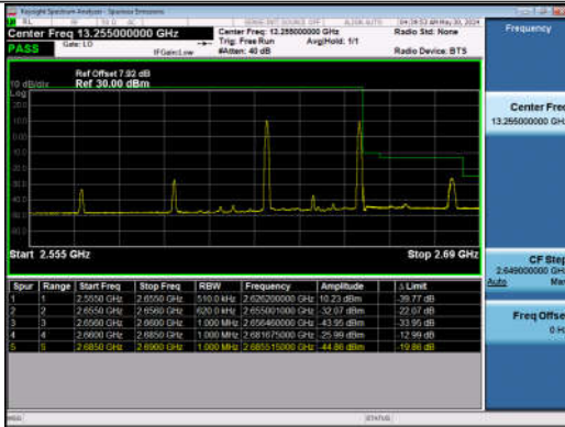
20MHz-10MHz_QPSK@QPSK-QPSK@QPSK_41041-41185_1RB#0@100RB#0-1RB#49@50RB#0
