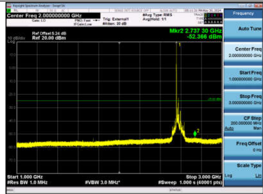
41-41-20MHz-20MHz-QPSK-QPSK-40340-40538-1RB#0-0 RB#0-1000~3000MHz-PASS
