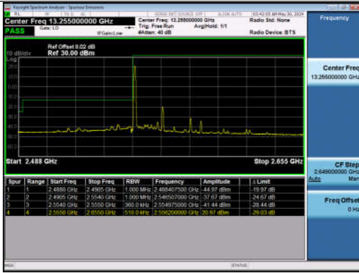
15MHz-20MHz_QPSK@QPSK-QPSK@QPSK_40318-40489_1RB#0@75RB#0-0RB#0@100RB#0
