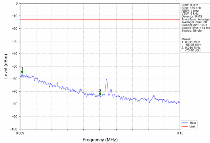
Band12_1.4MHz_QPSK_LCH_699.7MHz_RB_1_0_NTNV
