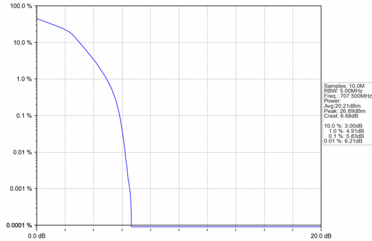
Band12_1.4MHz_16QAM_MCH_707.5MHz_RB_6_0_NTNV
