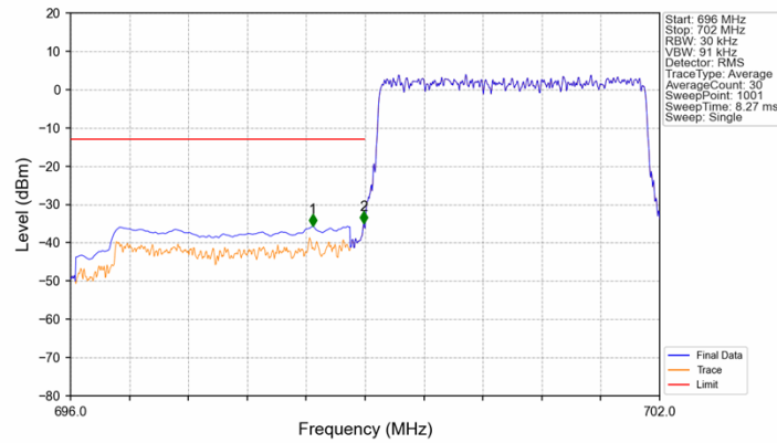
Band12_3MHz_QPSK_LCH_700.5MHz_RB_15_0_NTNV
