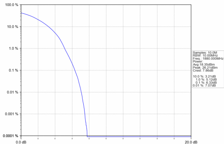
Band2 15MHz 16QAM MCH 1880MHz RB 75 0 NTV
