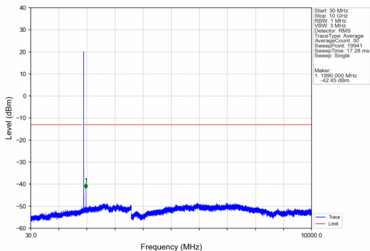
Band2_3MHz_16QAM_HCH_1908.5MHz_RB_1_0_NTNV
