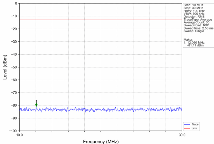
Band2_1.4MHz_16QAM_LCH_1850.7MHz_RB_1_0_NTNV
