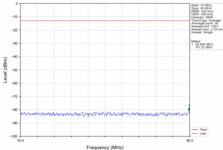
Band2_15MHz_16QAM_LCH_1857.5MHz_RB_1_0_NTNV
