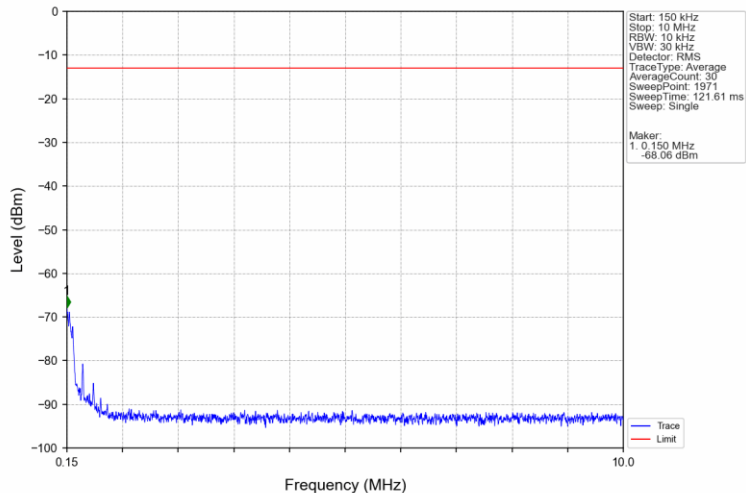
Band2_5MHz_16QAM_HCH_1907.5MHz_RB_1_0_NTNV
