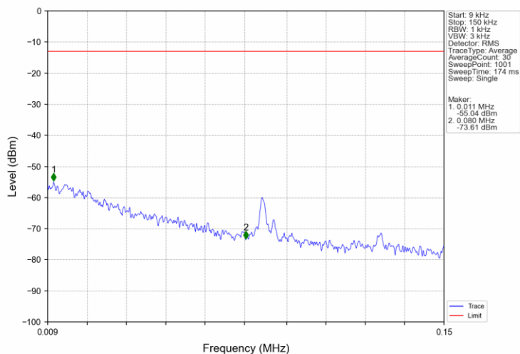
Band2_15MHz_16QAM_LCH_1857.5MHz_RB_1_0_NTNV
