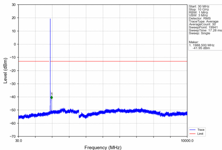
Band2_5MHz_16QAM_HCH_1907.5MHz_RB_1_0_NTNV
