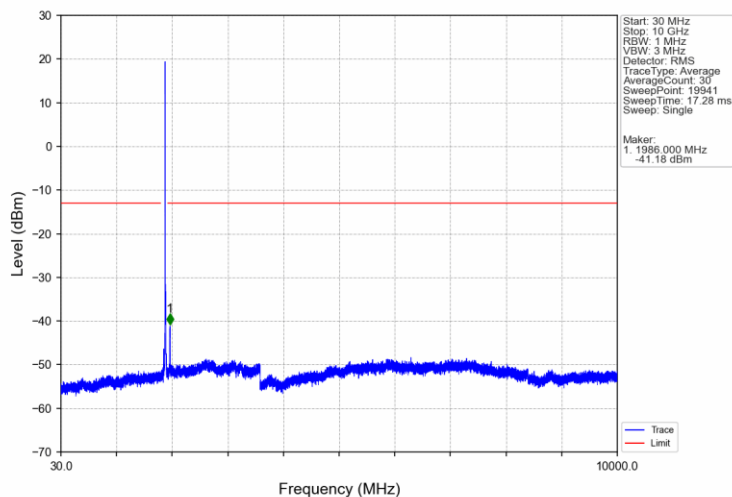
Band2_15MHz_16QAM_HCH_1902.5MHz_RB_1_0_NTNV
