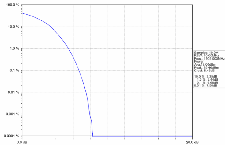
Band25_20MHz_16QAM_HCH_1905MHz_RB_100_0_NTNV
