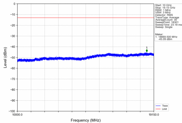
Band25_3MHz_QPSK_LCH_1851.5MHz_RB_1_0_NTNV
