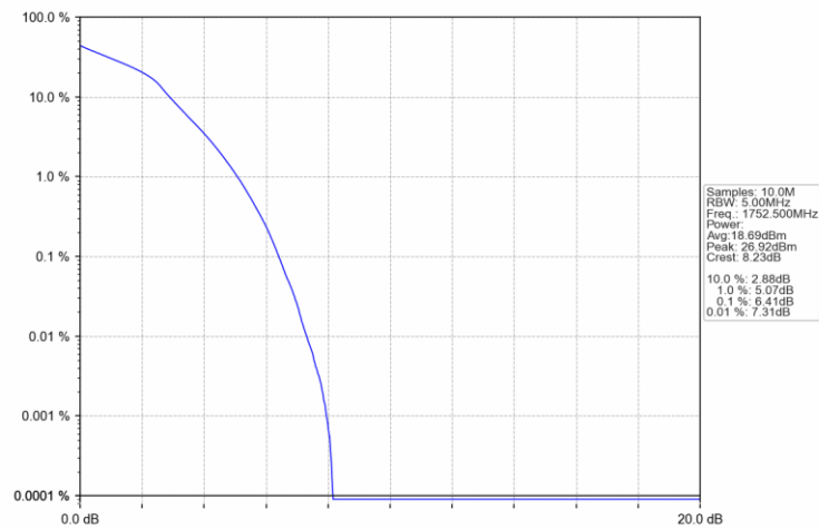
Band4 5MHz 16QAM HCH 1752.5MHz RB 25 0 NTV
