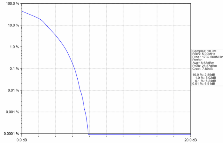
Band4 5MHz 16QAM MCH 1732.5MHz RB 25 0 NTV
