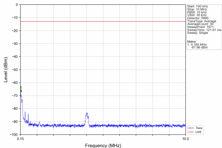
Band4_3MHz_QPSK_LCH_1711.5MHz_RB_1_0_NTNV
