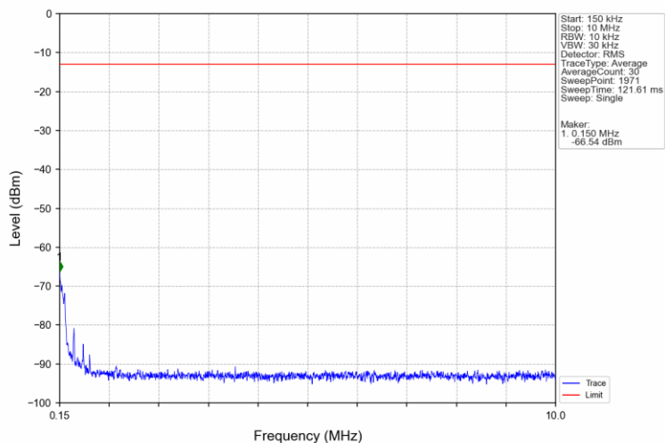
Band4_3MHz_QPSK_MCH_1732.5MHz_RB_1_0_NTNV
