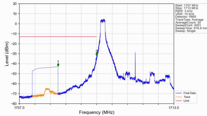
Band4_3MHz_QPSK_LCH_1711.5MHz_RB_1_0_NTNV
