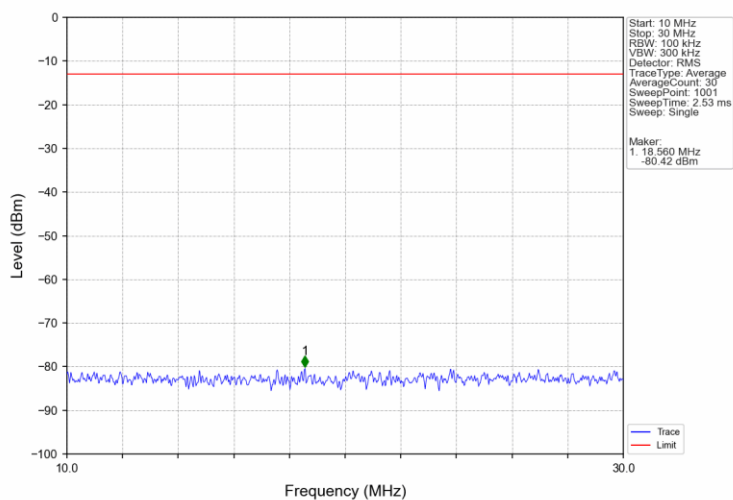
Band4_3MHz_QPSK_MCH_1732.5MHz_RB_1_0_NTNV
