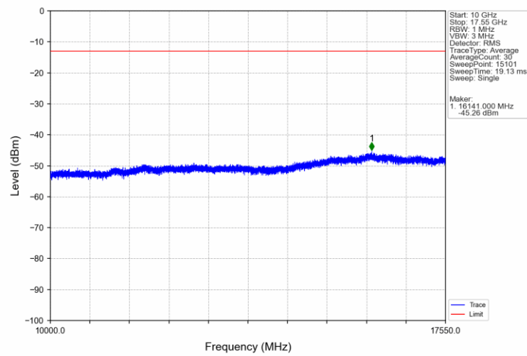
Band4_3MHz_16QAM_HCH_1753.5MHz_RB_1_0_NTNV
