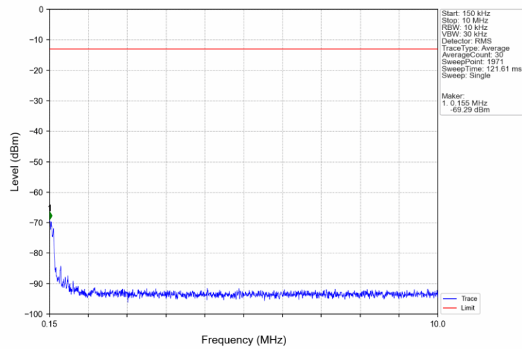
Band4 1.4MHz 16QAM MCH 1732.5MHz RB 1 0 NTNV
