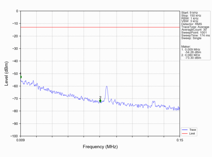
Band4_20MHz_16QAM_MCH_1732.5MHz_RB_1_0_NTNV
