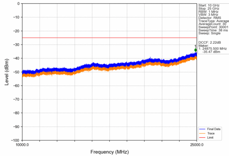
Band41 5MHz 16QAM MCH 2593MHz RB 1 0 NTNV
