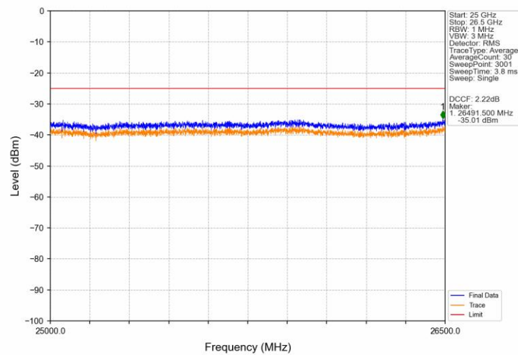
Band41 5MHz 16QAM HCH 2687.5MHz RB 1 0 NTNV
