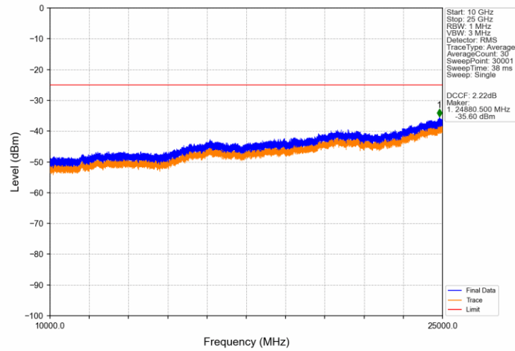
Band41 5MHz 16QAM HCH 2687.5MHz RB 1 0 NTNV
