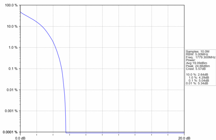
Band66 1.4MHz QPSK HCH 1779.3MHz RB 6 0 NTNV
