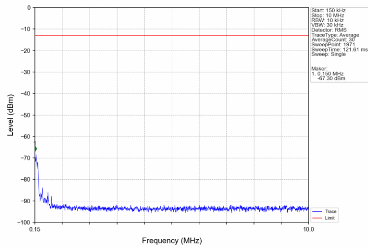
Band66 3MHz 16QAM MCH 1745MHz RB 1 0 NTV
