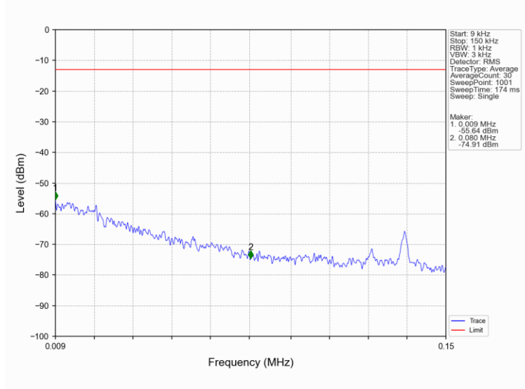
Band66_3MHz_16QAM_LCH_1711.5MHz_RB_1_0_NTNV
