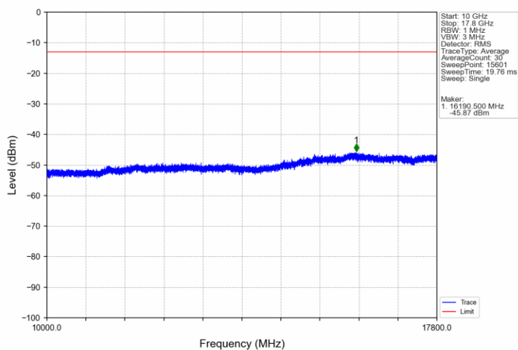
Band66 5MHz QPSK MCH 1745MHz RB 1 0 NTNV
