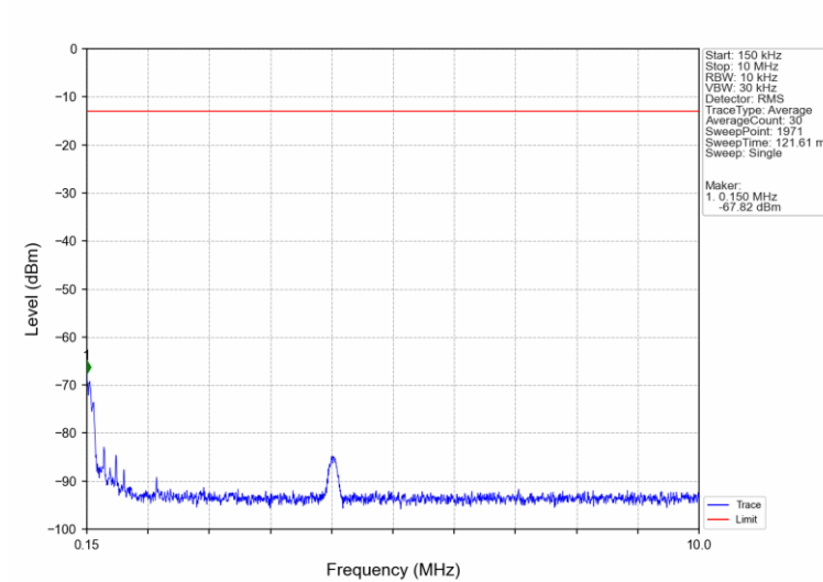
Band66_3MHz_16QAM_LCH_1711.5MHz_RB_1_0_NTNV
