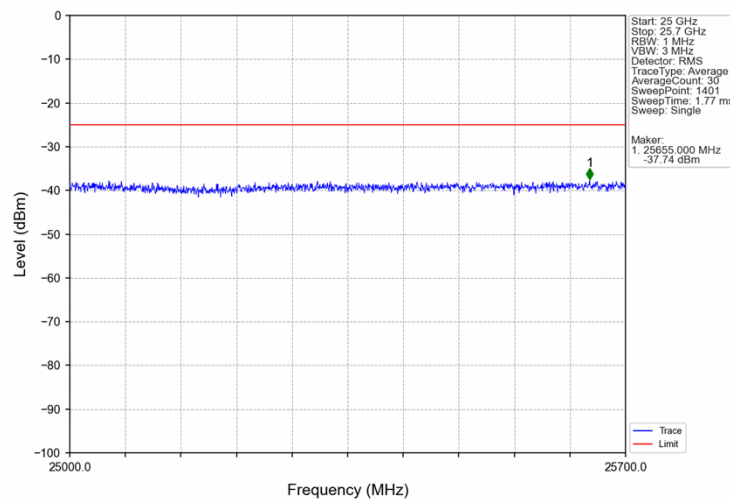
Band7 15MHz QPSK MCH 2535MHz RB 1 0 NTNV
