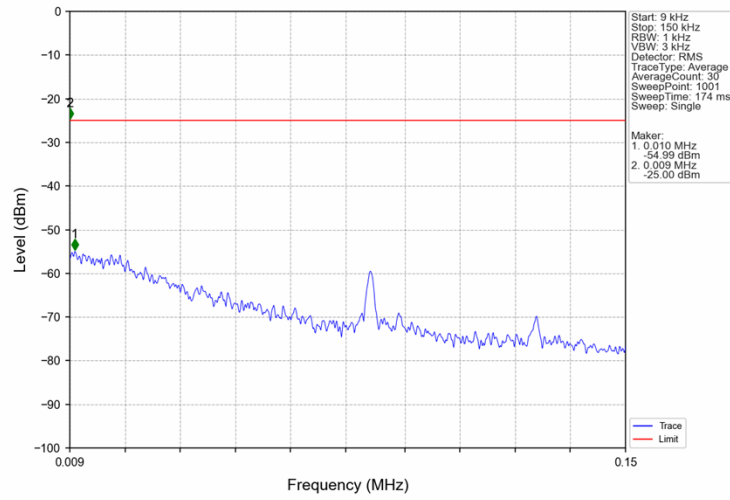
Band7 15MHz 16QAM HCH 2562.5MHz RB 1 0 NTNV
