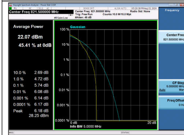
Band26(Part 90)-5MHz-16QAM-26765-1RB#0-PASS
