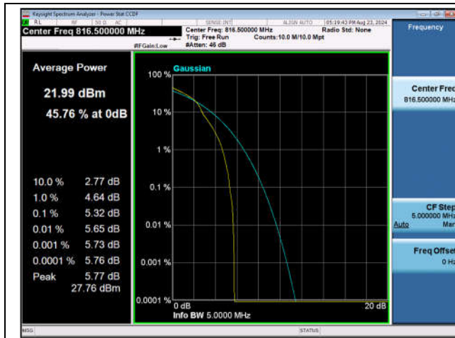
Band26(Part 90)-5MHz-16QAM-26715-1RB#0-PASS
