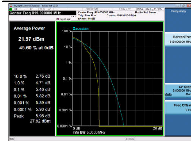
Band26(Part 90)-5MHz-16QAM-26740-1RB#0-PASS
