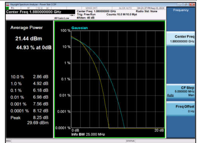
Band2-20MHz-16QAM-18900-100RB#0-PASS
