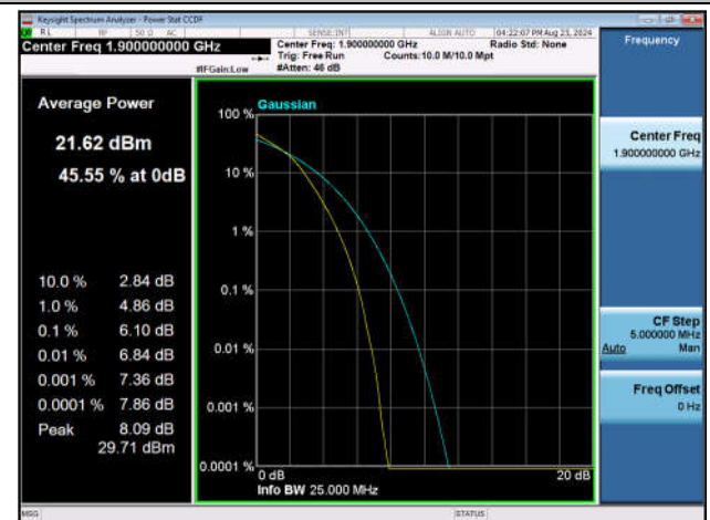
Band2-20MHz-16QAM-19100-100RB#0-PASS
