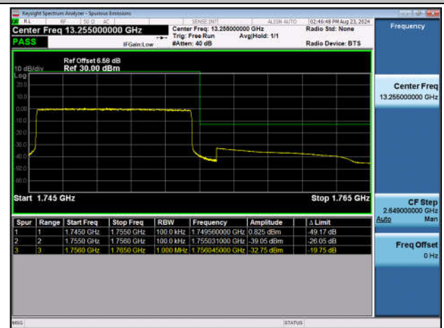
Band4_10MHz_QPSK_20350_50RB#0
