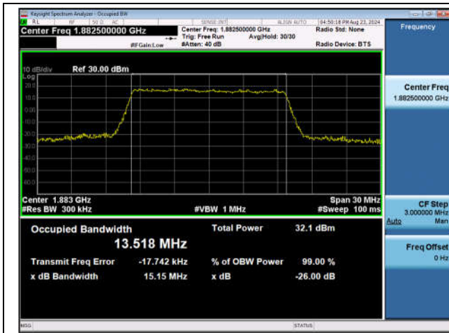
Band25-15MHz-QPSK-26365-75RB#0-PASS
