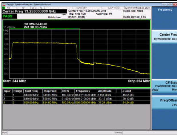
Band5_5MHz_QPSK_20625_25RB#0
