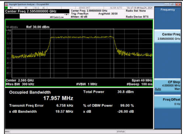
Band38-20MHz-16QAM-38000-100RB#0-PASS
