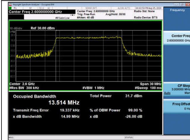
Band41-15MHz-QPSK-40690-75RB#0-PASS
