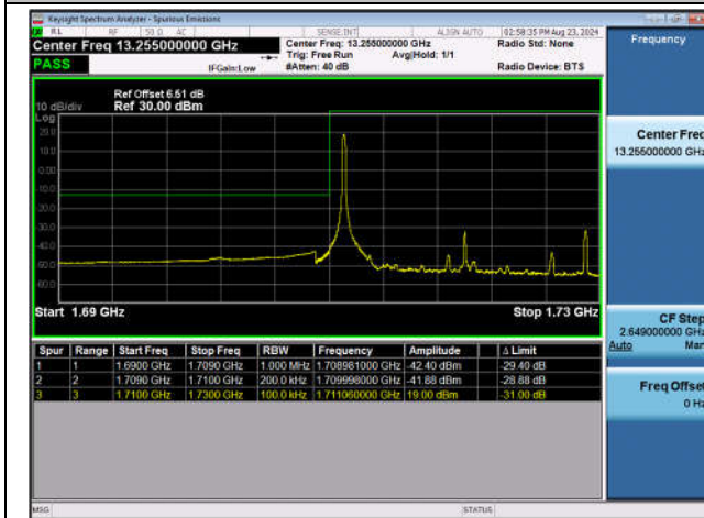
Band4_20MHz_QPSK_20050_1RB#0
