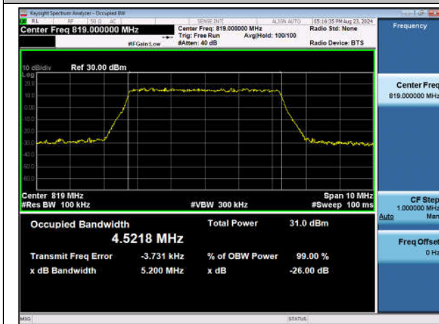
Band26(Part 90)-5MHz-QPSK-26740-25RB#0-PASS
