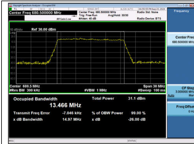
Band71-15MHz-QPSK-133297-75RB#0-PASS
