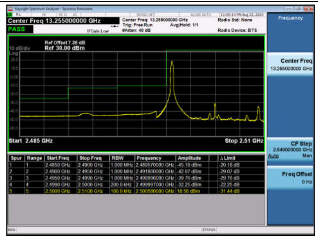
Band7_10MHz_QPSK_20800_1RB#0
