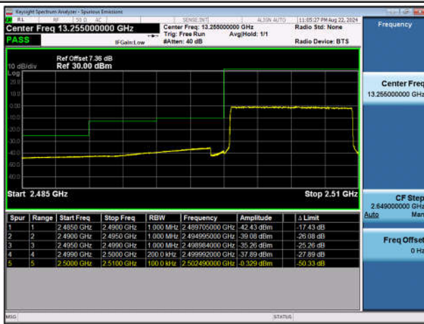
Band7_10MHz_QPSK_20800_50RB#0
