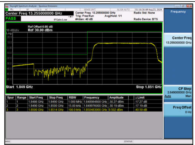
Band2_1.4MHz_QPSK_18607_6RB#0
