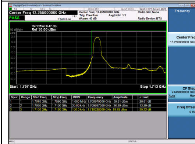
Band4_3MHz_QPSK_19965_1RB#0
