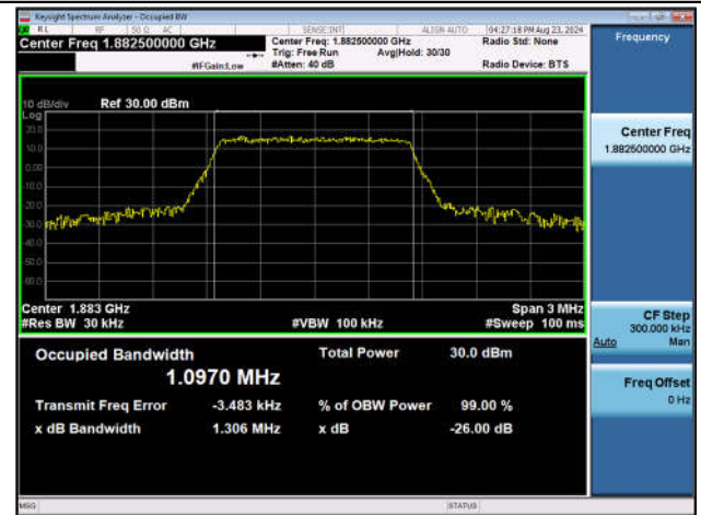
Band25-1.4MHz-16QAM-26365-6RB#0-PASS
