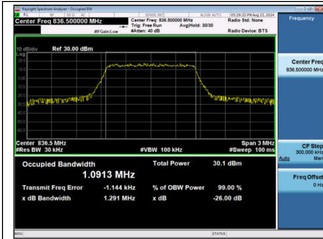
Band26(Part 22)-1.4MHz-QPSK-26915-6RB#0-PASS
