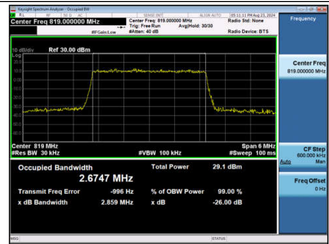
Band26(Part 90)-3MHz-16QAM-26740-15RB#0-PASS
