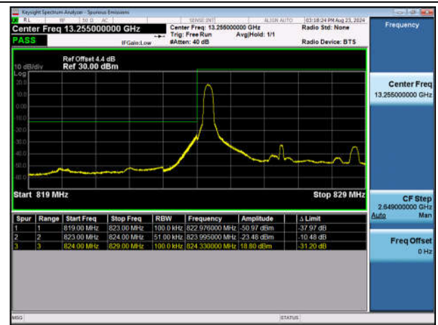
Band5_5MHz_QPSK_20425_1RB#0
