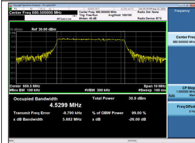
Band71-5MHz-QPSK-133297-25RB#0-PASS
