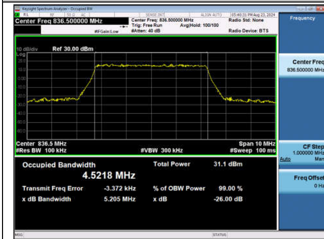
Band26(Part 22)-5MHz-QPSK-26915-25RB#0-PASS
