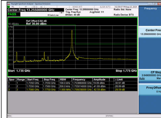
Band4_20MHz_QPSK_20300_1RB#99
