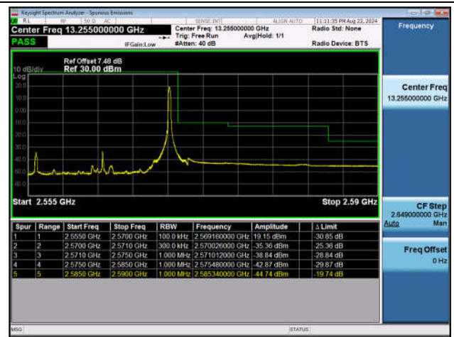
Band7_15MHz_QPSK_21375_1RB#74
