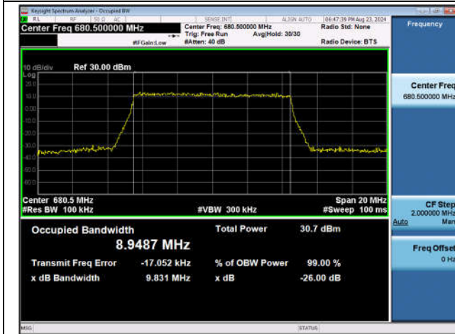
Band71-10MHz-QPSK-133297-50RB#0-PASS
