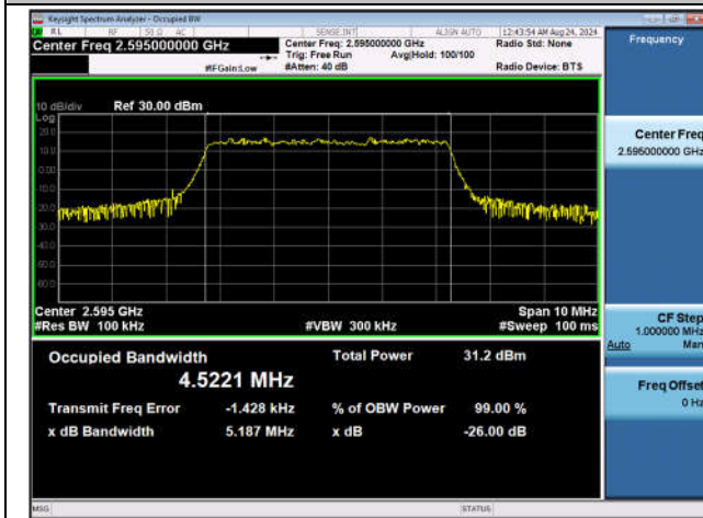
Band38-5MHz-QPSK-38000-25RB#0-PASS
