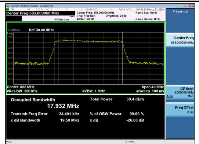
Band71-20MHz-16QAM-133322-100RB#0-PASS
