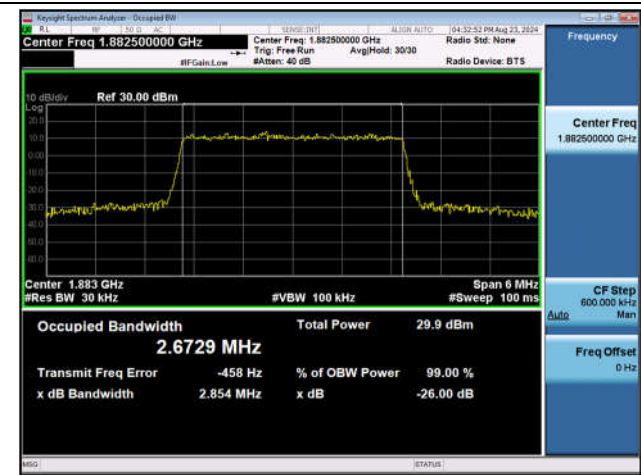
Band25-3MHz-16QAM-26365-15RB#0-PASS
