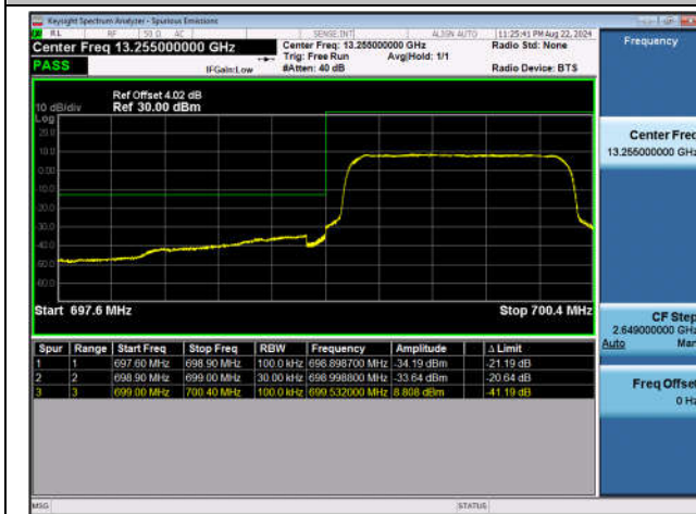
Band12_1.4MHz_QPSK_23017_6RB#0
