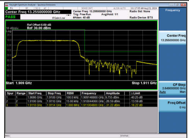
Band2_1.4MHz_QPSK_19193_6RB#0
