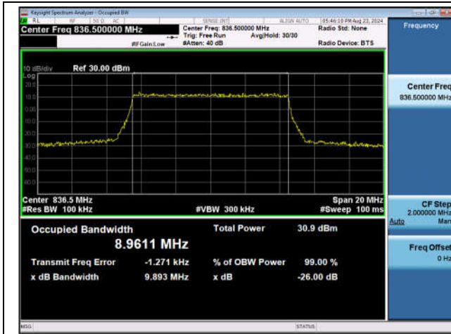
Band26(Part 22)-10MHz-QPSK-26915-50RB#0-PASS
