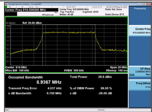
Band26(Part 90)-10MHz-16QAM-26740-50RB#0-PASS
