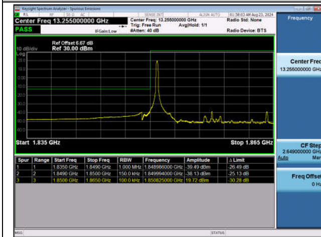
Band2_15MHz_QPSK_18675_1RB#0
