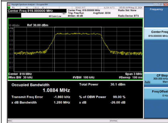
Band26(Part 90)-1.4MHz-QPSK-26740-6RB#0-PASS
