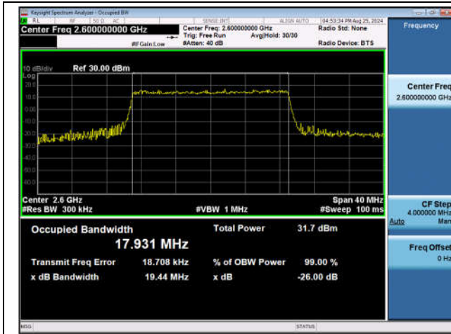
Band41-20MHz-QPSK-40690-100RB#0-PASS
