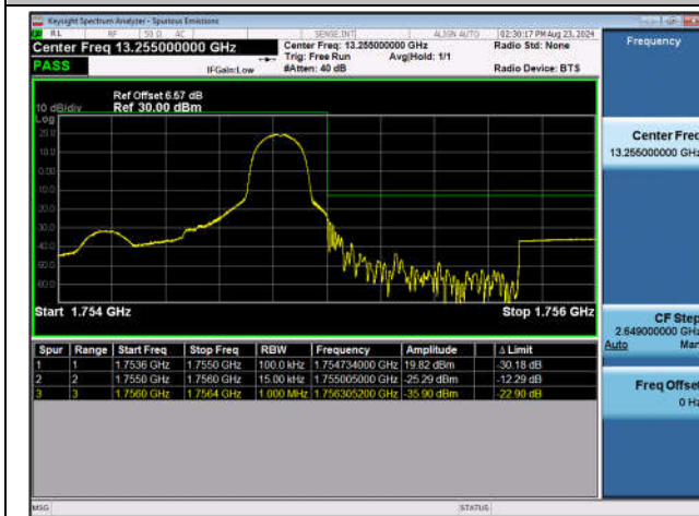
Band4_1.4MHz_QPSK_20393_1RB#5
