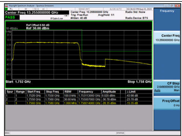
Band4_3MHz_QPSK_20385_15RB#0
