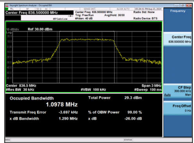
Band26(Part 22)-1.4MHz-16QAM-26915-6RB#0-PASS
