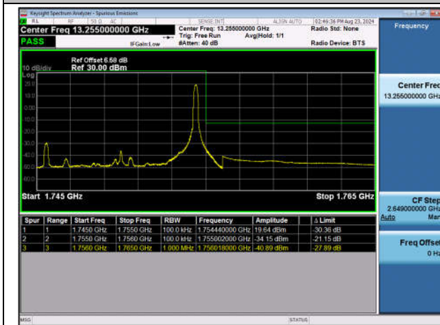
Band4_10MHz_QPSK_20350_1RB#49
