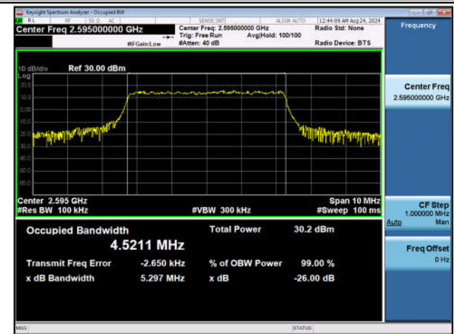
Band38-5MHz-16QAM-38000-25RB#0-PASS
