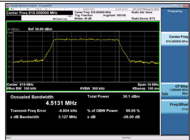
Band26(Part 90)-5MHz-16QAM-26740-25RB#0-PASS
