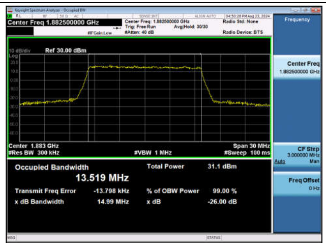
Band25-15MHz-16QAM-26365-75RB#0-PASS
