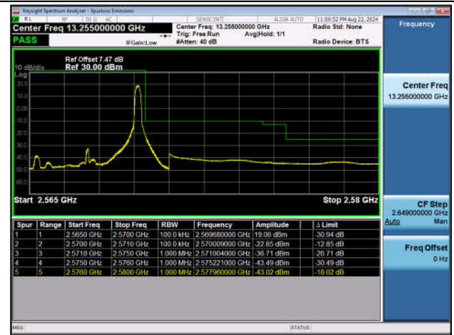
Band7_5MHz_QPSK_21425_1RB#24
