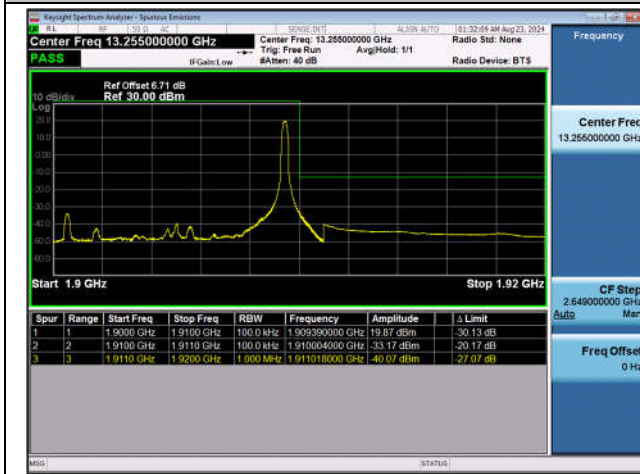
Band2_10MHz_QPSK_19150_1RB#49
