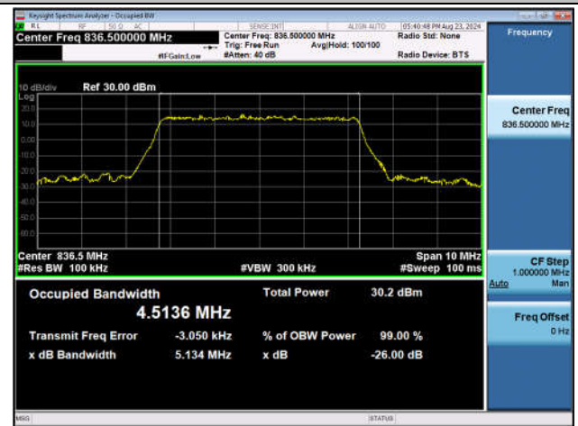
Band26(Part 22)-5MHz-16QAM-26915-25RB#0-PASS
