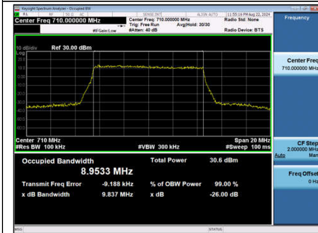
Band17-10MHz-QPSK-23790-50RB#0-PASS
