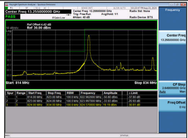
Band5_10MHz_QPSK_20450_1RB#0
