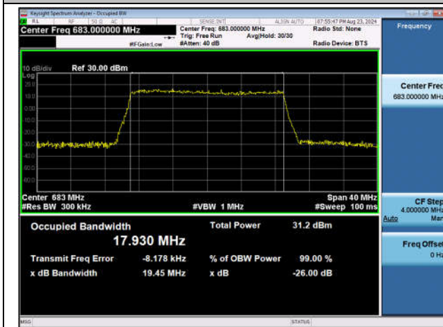
Band71-20MHz-QPSK-133322-100RB#0-PASS
