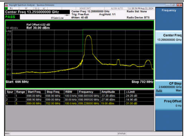
Band12_3MHz_QPSK_23025_1RB#0
