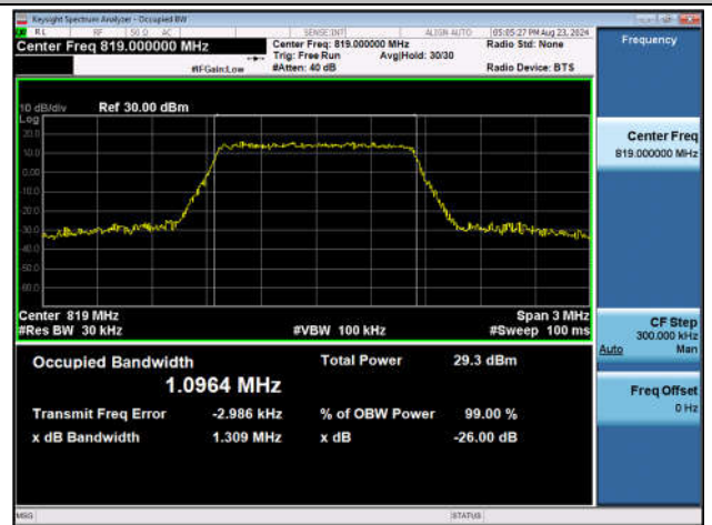
Band26(Part 90)-1.4MHz-16QAM-26740-6RB#0-PASS
