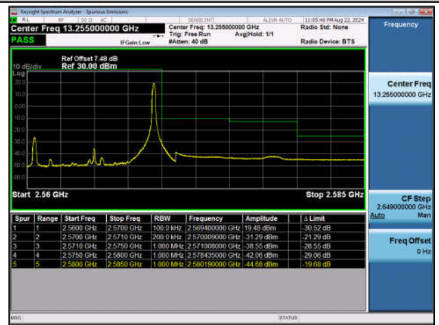
Band7_10MHz_QPSK_21400_1RB#49
