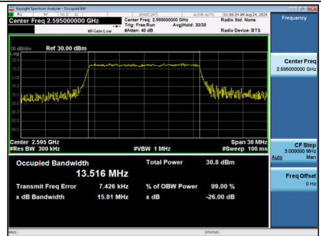
Band38-15MHz-16QAM-38000-75RB#0-PASS
