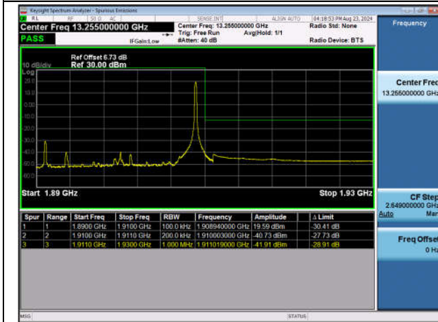
Band2_20MHz_QPSK_19100_1RB#99
