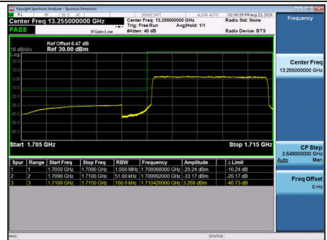
Band4_5MHz_QPSK_19975_25RB#0
