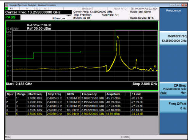
Band7_5MHz_QPSK_20775_1RB#0
