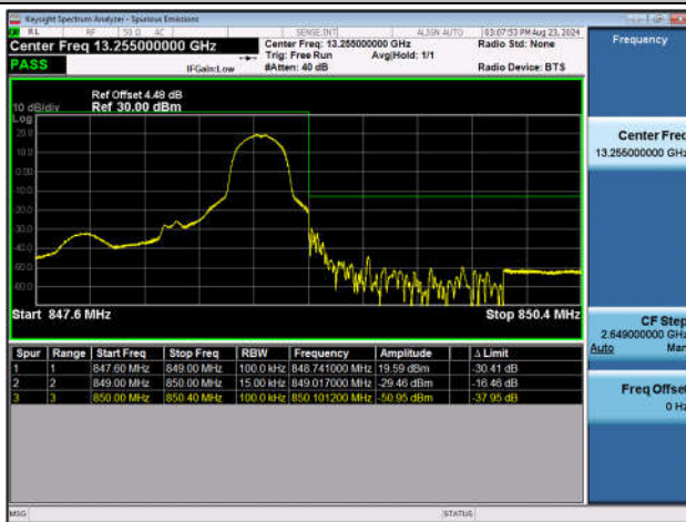
Band5_1.4MHz_QPSK_20643_1RB#5
