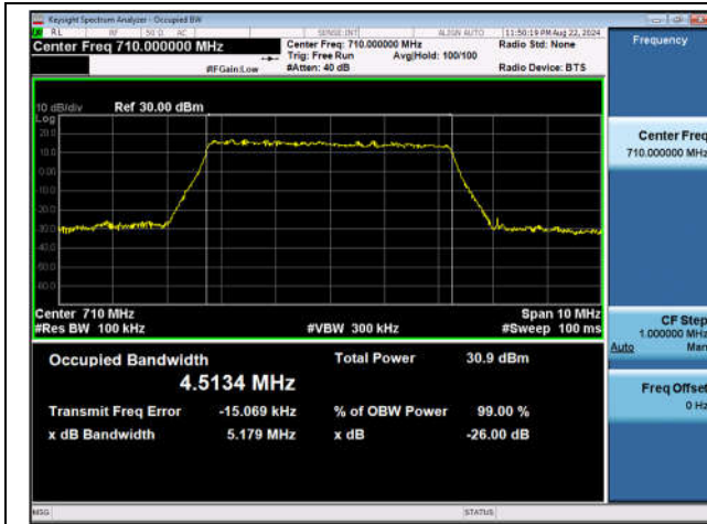
Band17-5MHz-QPSK-23790-25RB#0-PASS
