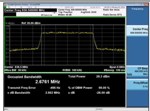
Band26(Part 22)-3MHz-16QAM-26915-15RB#0-PASS
