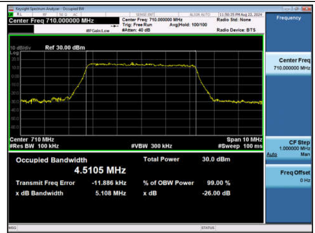
Band17-5MHz-16QAM-23790-25RB#0-PASS
