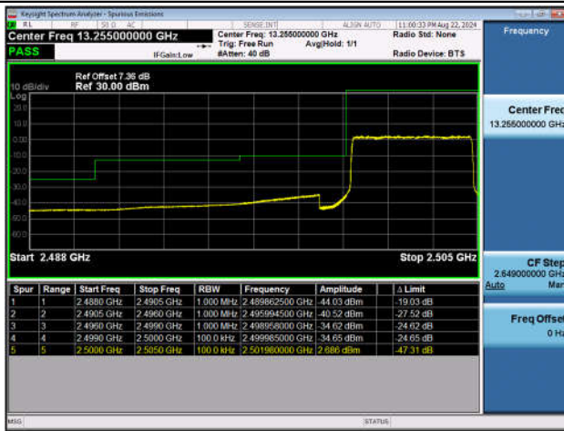
Band7_5MHz_QPSK_20775_25RB#0
