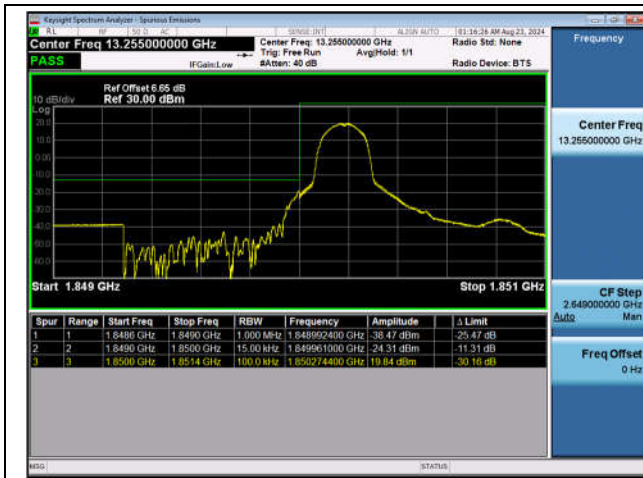
Band2_1.4MHz_QPSK_18607_1RB#0
