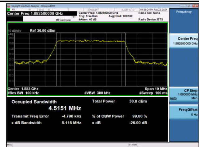
Band25-5MHz-16QAM-26365-25RB#0-PASS
