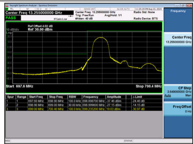
Band12_1.4MHz_QPSK_23017_1RB#0
