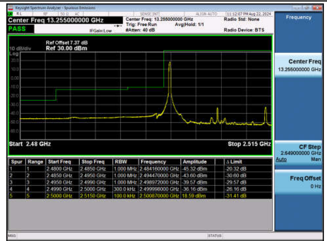
Band7_15MHz_QPSK_20825_1RB#0
