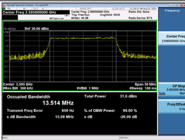
Band38-15MHz-QPSK-38000-75RB#0-PASS
