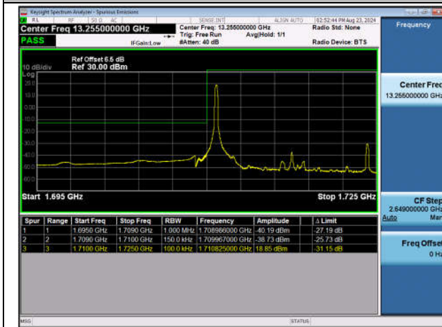
Band4_15MHz_QPSK_20025_1RB#0
