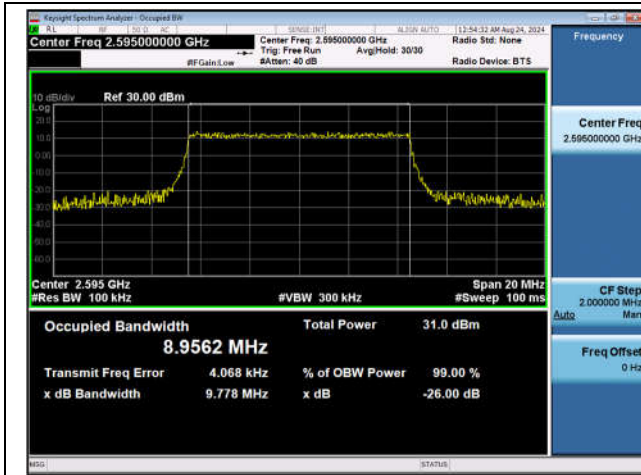
Band38-10MHz-QPSK-38000-50RB#0-PASS
