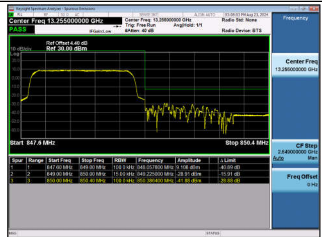
Band5_1.4MHz_QPSK_20643_6RB#0
