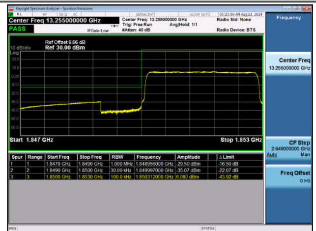
Band2_3MHz_QPSK_18615_15RB#0
