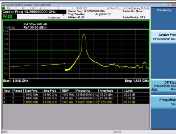
Band2_5MHz_QPSK_18625_1RB#0
