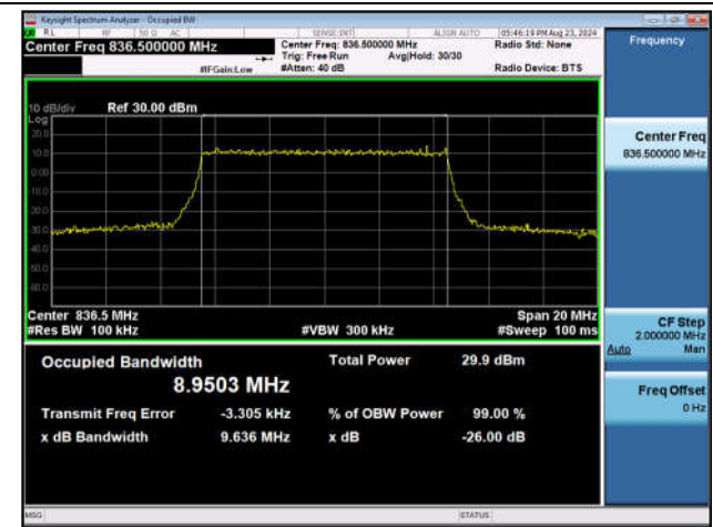
Band26(Part 22)-10MHz-16QAM-26915-50RB#0-PASS
