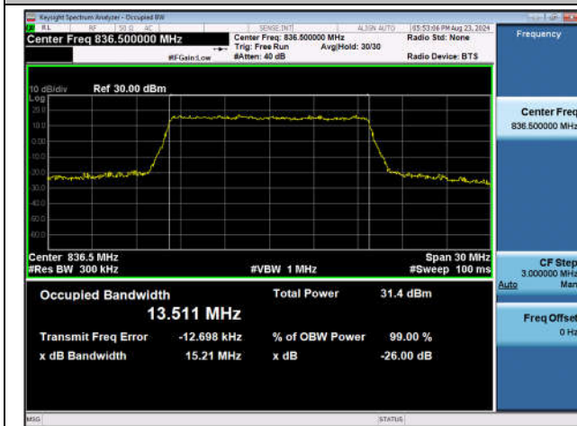
Band26(Part 22)-15MHz-QPSK-26915-75RB#0-PASS
