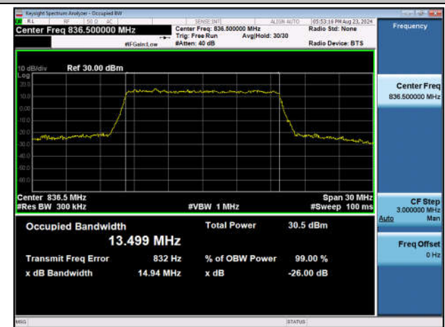
Band26(Part 22)-15MHz-16QAM-26915-75RB#0-PASS
