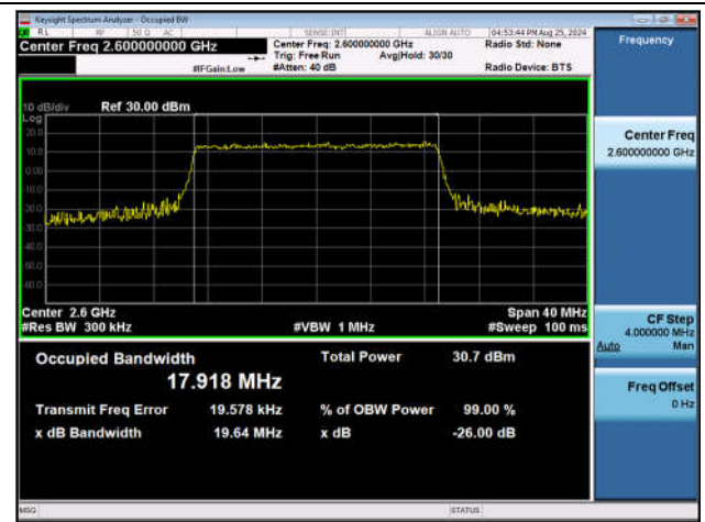
Band41-20MHz-16QAM-40690-100RB#0-PASS
