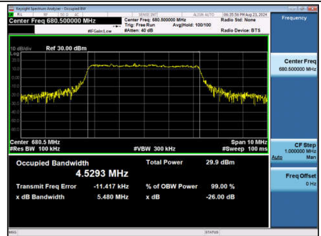
Band71-5MHz-16QAM-133297-25RB#0-PASS
