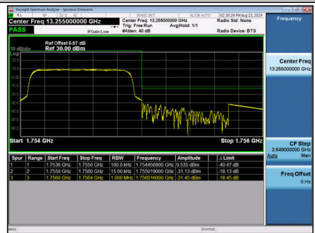
Band4_1.4MHz_QPSK_20393_6RB#0
