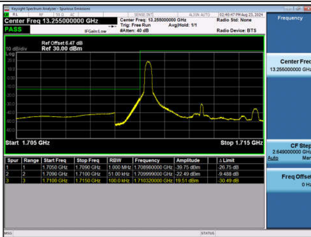
Band4_5MHz_QPSK_19975_1RB#0
