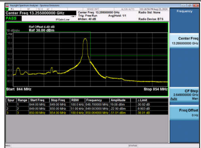
Band5_5MHz_QPSK_20625_1RB#24
