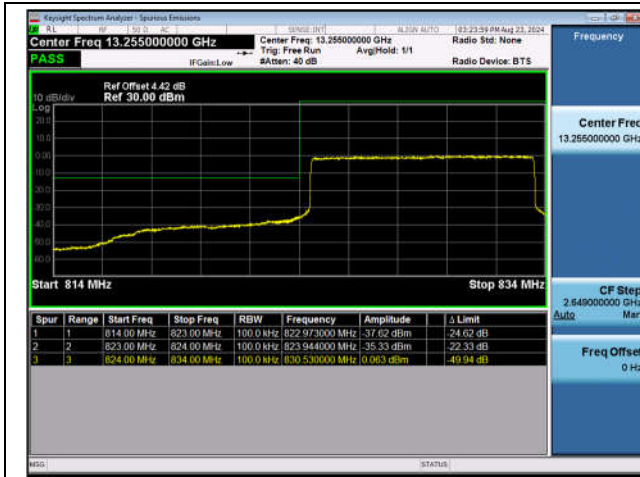
Band5_10MHz_QPSK_20450_50RB#0
