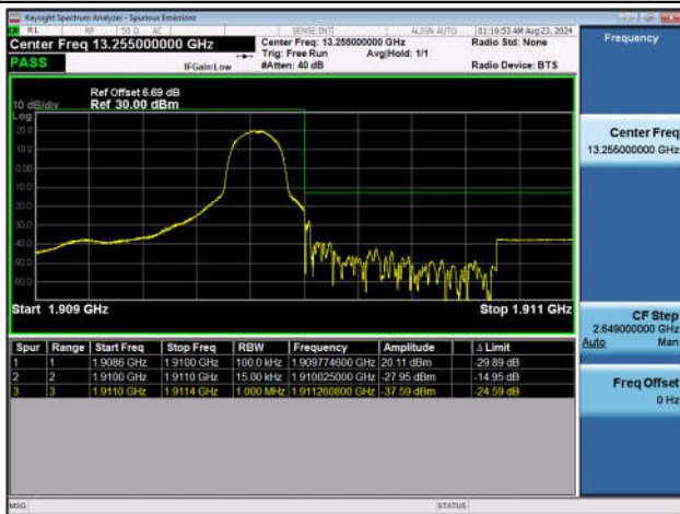
Band2_1.4MHz_QPSK_19193_1RB#5
