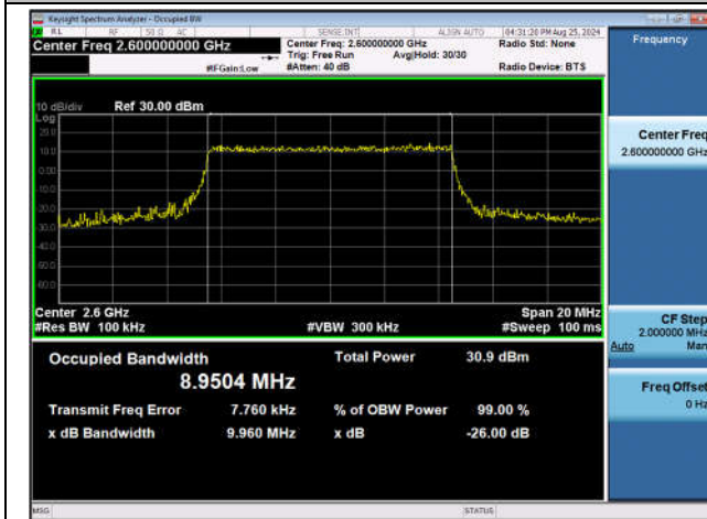
Band41-10MHz-QPSK-40690-50RB#0-PASS
