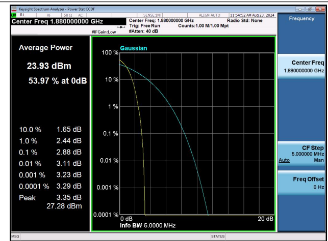
Band2-9400-PASS
