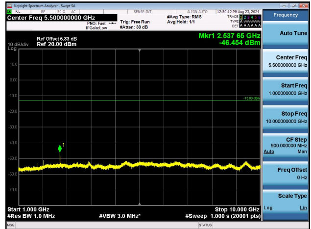
Band5-4233-1000~10000MHz-PASS
