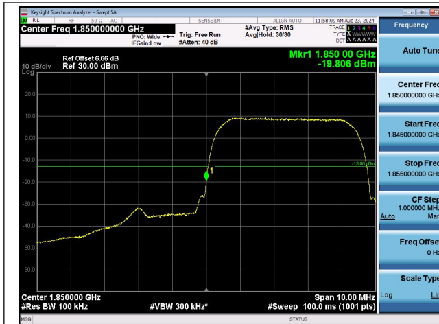
Band2-9262-PASS
