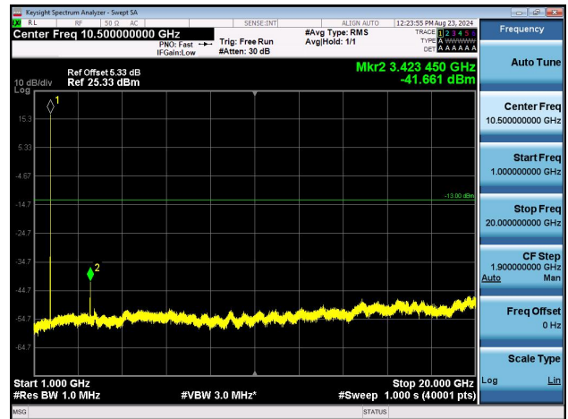
Band4-1312-1000~20000MHz-PASS
