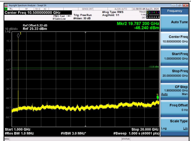
Band2-9262-1000~20000MHz-PASS
