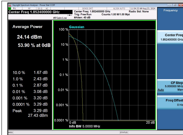
Band2-9262-PASS
