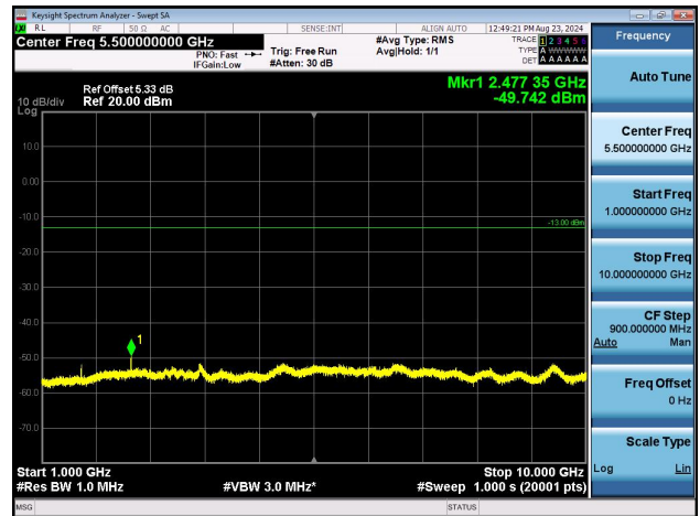
Band5-4132-1000~10000MHz-PASS
