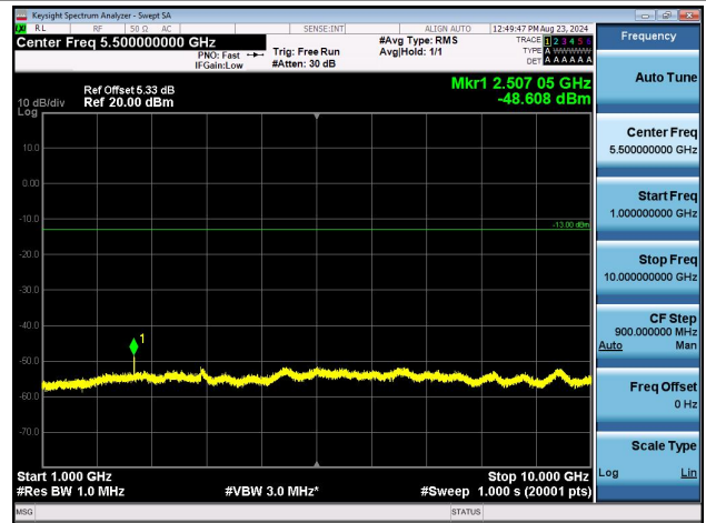
Band5-4183-1000~10000MHz-PASS
