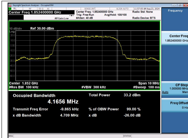
Band2-9262-PASS
