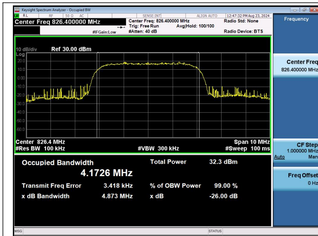
Band5-4132-PASS
