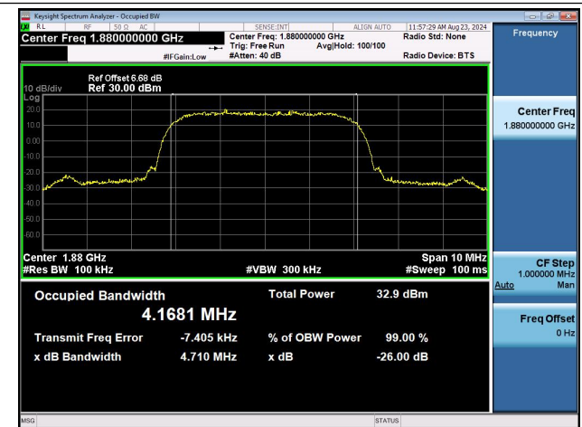
Band2-9400-PASS
