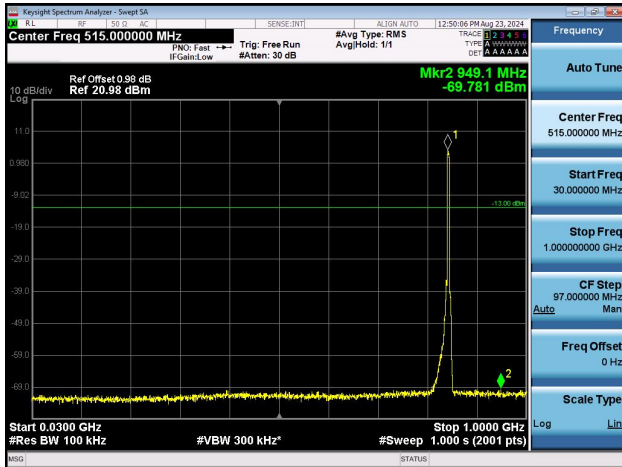
Band5-4233-30~1000MHz-PASS
