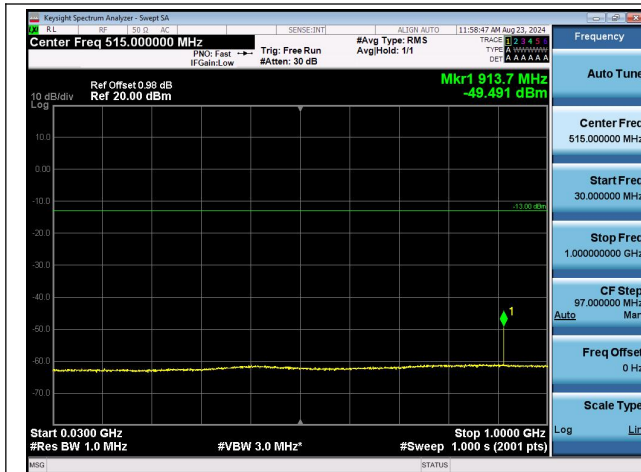
Band2-9262-30~1000MHz-PASS
