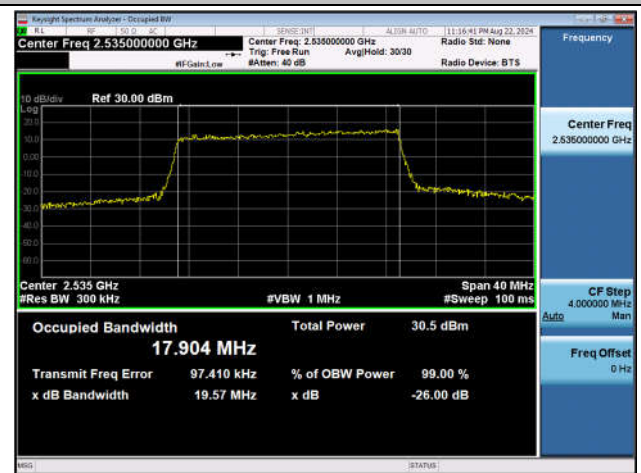
Band7-20MHz-16QAM-21100-100RB#0-PASS
