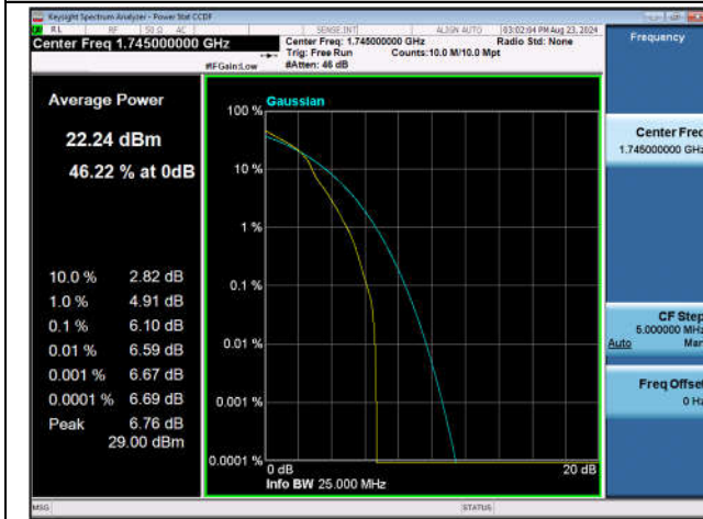
Band4-20MHz-16QAM-20300-1RB#0-PASS
