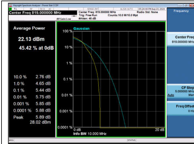
Band26(Part 90)-10MHz-16QAM-26740-1RB#0-PASS
