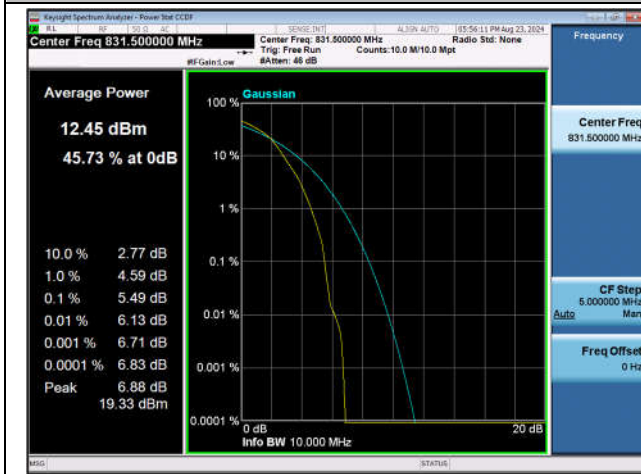
Band26(Part 22)-15MHz-16QAM-26865-1RB#0-PASS
