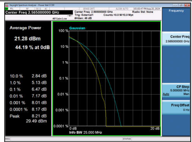
Band41-20MHz-16QAM-40340-100RB#0-PASS
