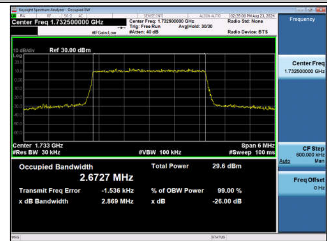
Band4-3MHz-16QAM-20175-15RB#0-PASS
