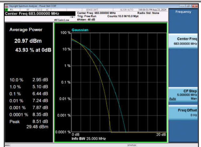
Band71-20MHz-16QAM-133322-100RB#0-PASS
