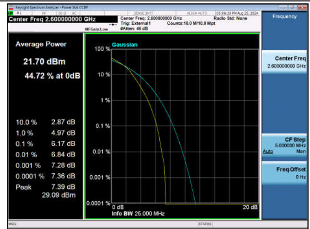
Band41-20MHz-16QAM-40690-100RB#0-PASS
