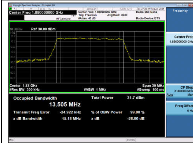
Band2-15MHz-QPSK-18900-75RB#0-PASS
