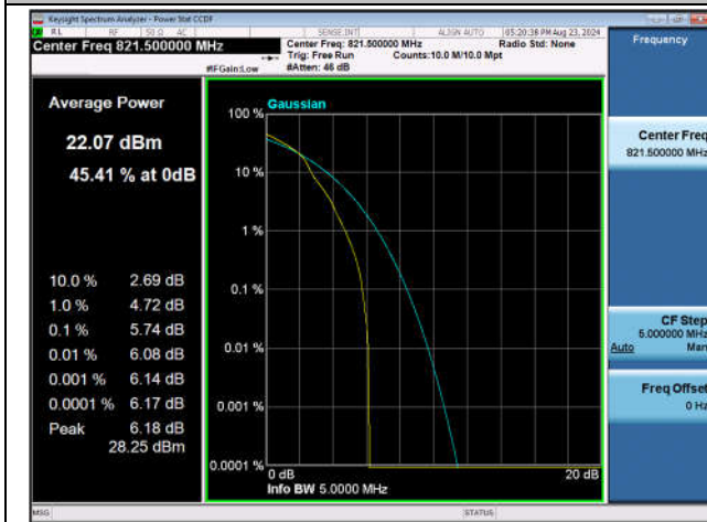
Band26(Part 90)-5MHz-16QAM-26765-1RB#0-PASS
