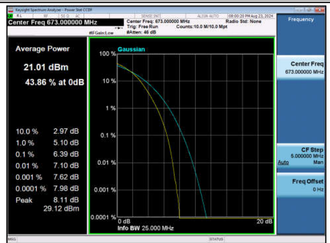
Band71-20MHz-16QAM-133222-100RB#0-PASS
