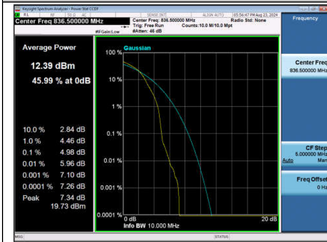
Band26(Part 22)-15MHz-16QAM-26915-1RB#0-PASS
