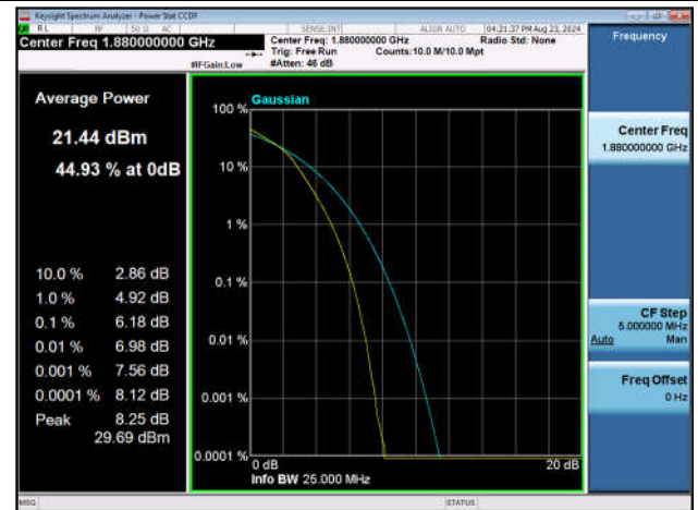
Band2-20MHz-16QAM-18900-100RB#0-PASS
