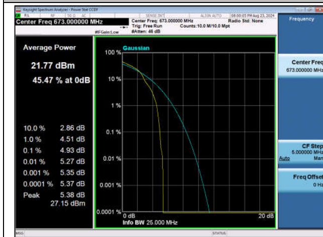
Band71-20MHz-16QAM-133222-1RB#0-PASS
