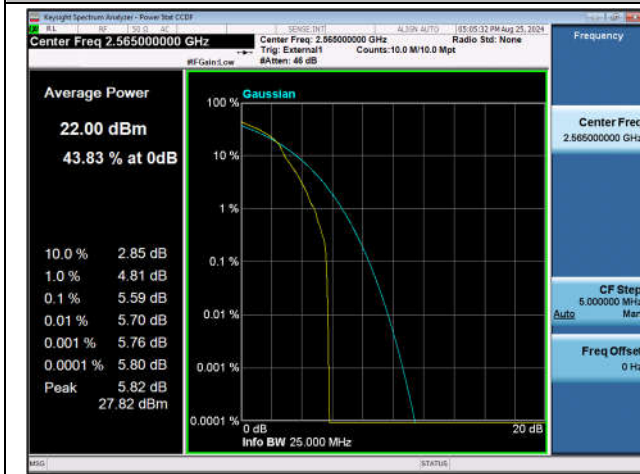
Band41-20MHz-16QAM-40340-1RB#0-PASS
