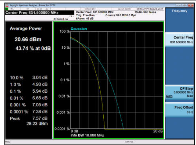
Band26(Part 22)-15MHz-16QAM-26865-75RB#0-PASS
