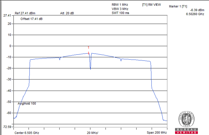
802.11ax (HE160) Beamforming / Chain 0 : CH 111
