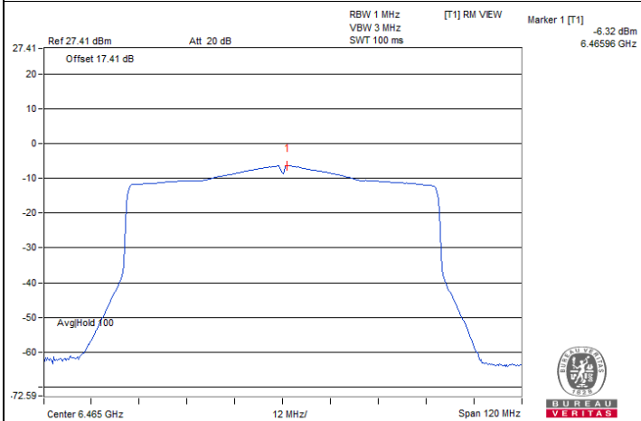
802.11ax (HE80) Beamforming / Chain 0 : CH 103
