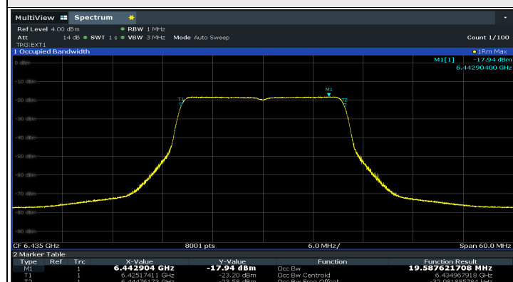
Plots of EUT Tx waveform
