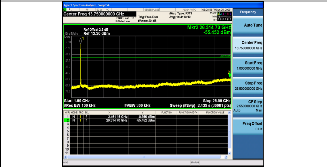
11AX20SISO_Ant1_2462_1000~26500
