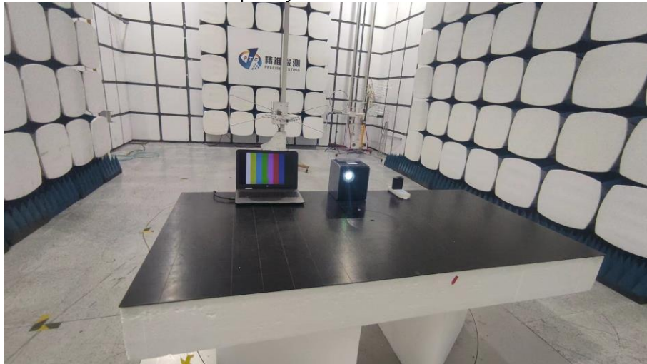
Radiated Spurious Emissions Test Frequency From 30MHz-1000MHz
