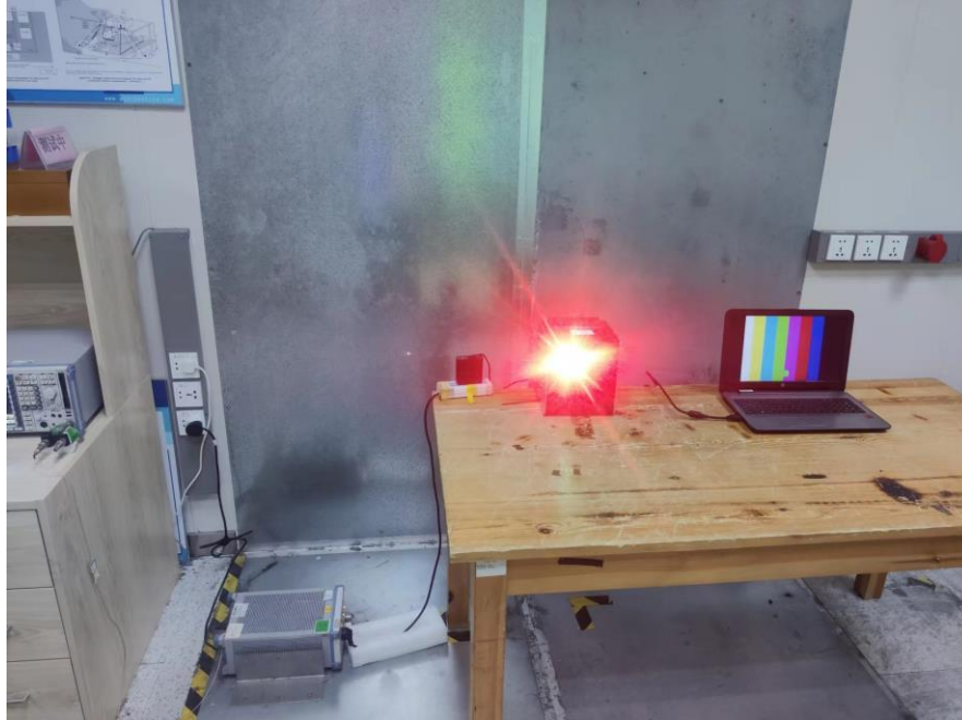
Conduction Emissions
