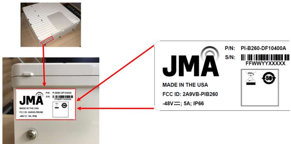
Figure 2 DUT Label Location
