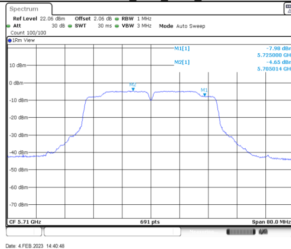
11AC40SISO_Ant1_5710_UNII-3
