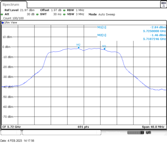
11AC20SISO Ant1 5720 UNII-3
