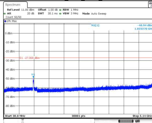
11N40SISO Ant1 5230 30-5140
