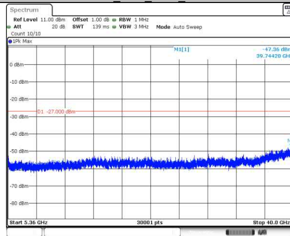
11N40SISO Ant1 5190 5360-40000
