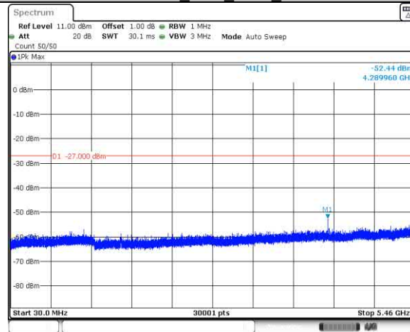
11AC20SISO Ant1 5720 30~5460
