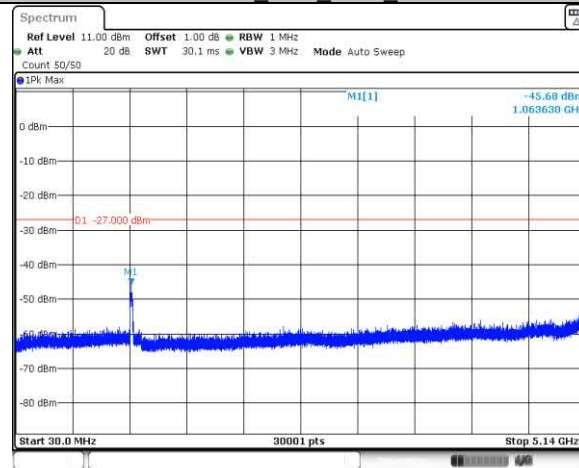
11AC40SISO Ant1 5270 30~5140
