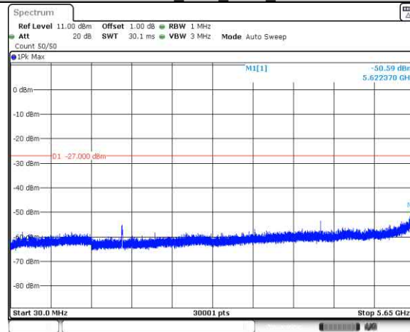
11N20SISO Ant1 5785 30-5650
