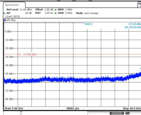
11AC40SISO Ant1 5230 5360~40000
