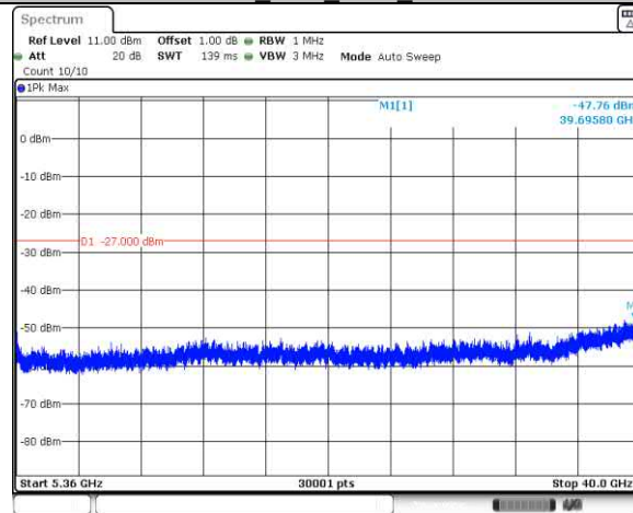
11AC20SISO Ant1 5320 5360~40000
