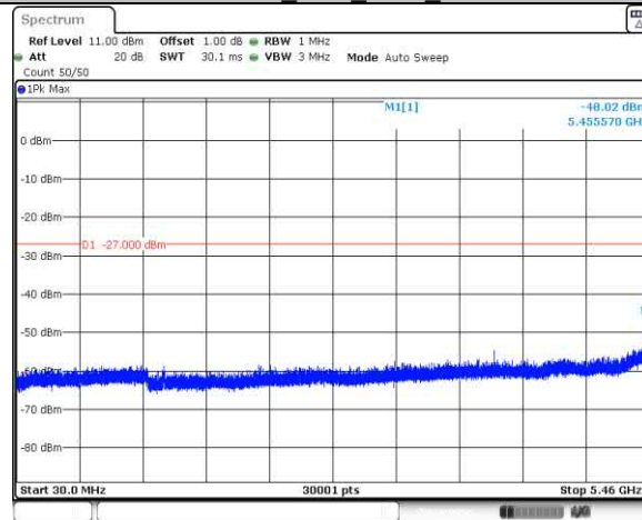
11AC20SISO Ant1 5500 30~5460
