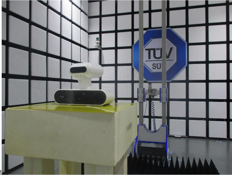
18G-40GHz RSE Setup
