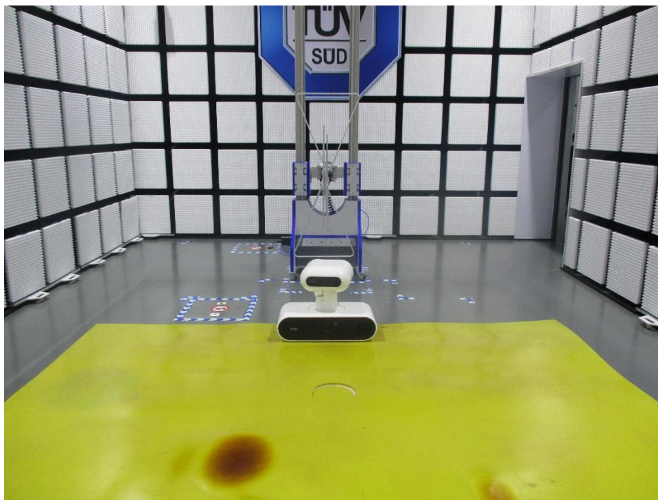
30M-1000MHz RSE Setup
