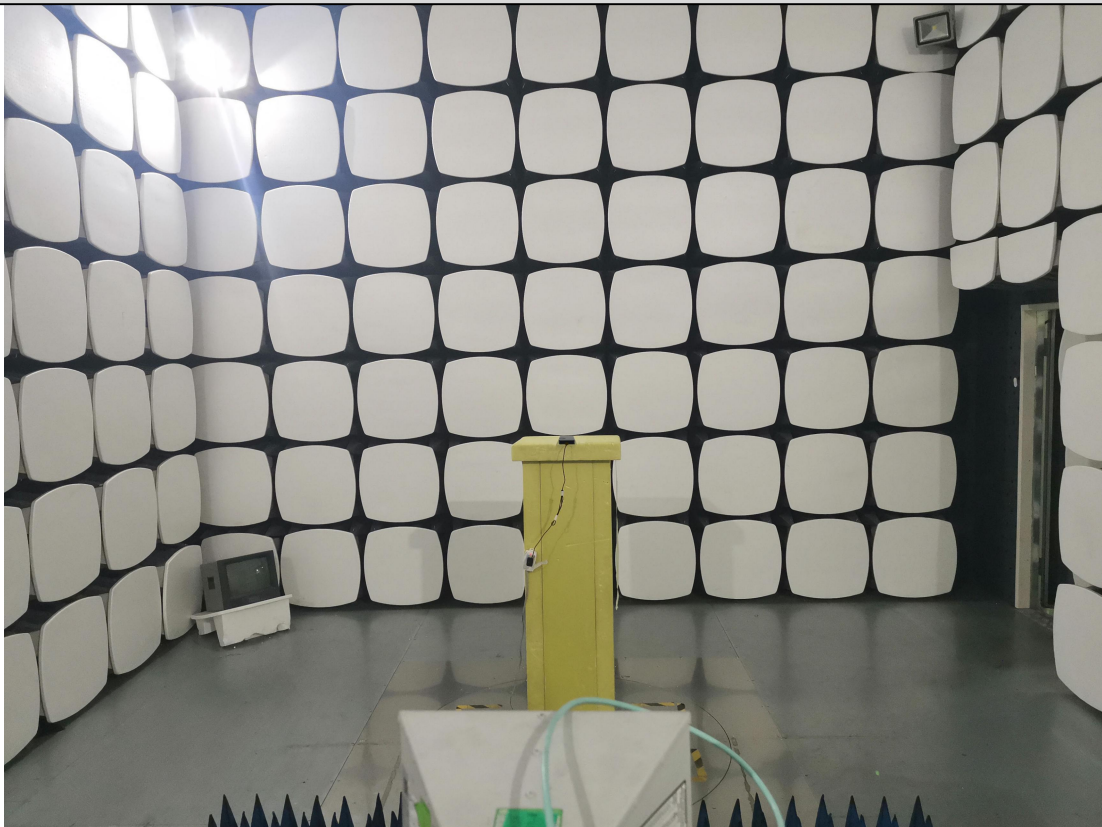
RE above 1G Test Setup
