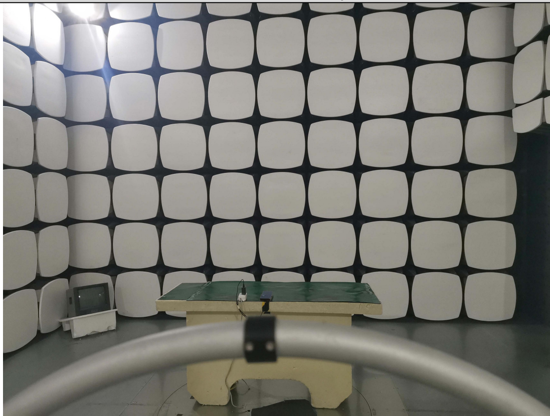
RE 9k-30M Test Setup
