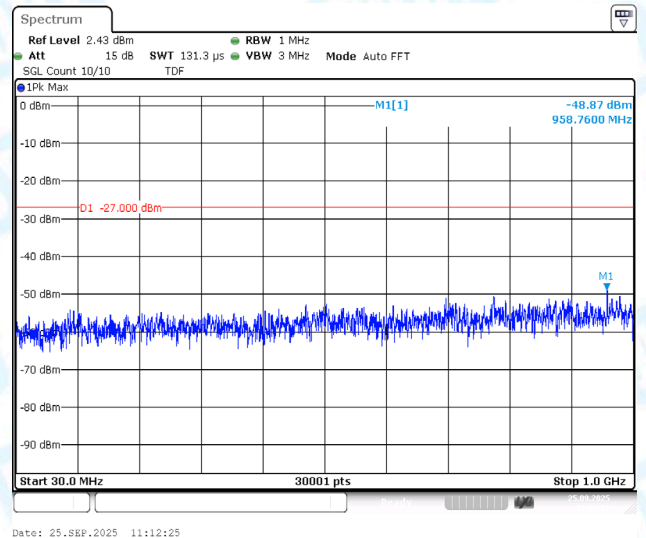
11AC20MIMO-Ant2-5240-30~1000-PASS
