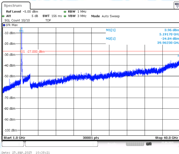
11N40MIMO-Ant1-5190-1000~40000-PASS
