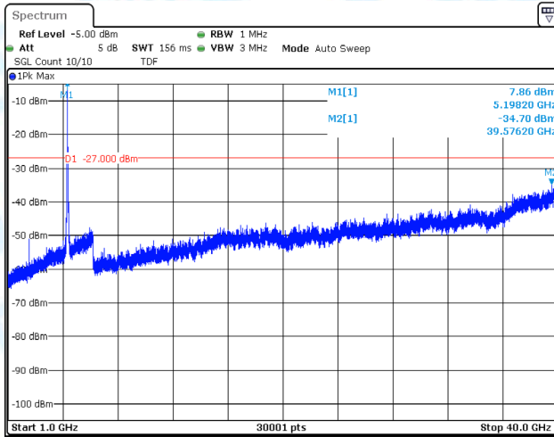
11A-CDD-Ant1-5200-1000~40000-PASS
