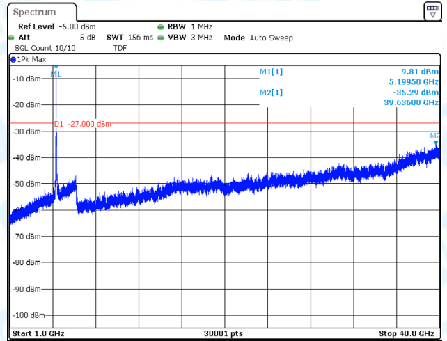
11A-CDD-Ant2-5200-1000~40000-PASS
