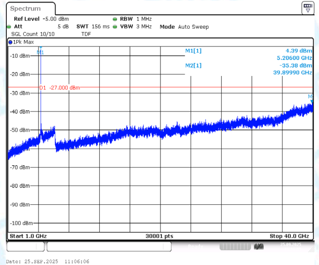
11AC20MIMO-Ant2-5200-1000~40000-PASS
