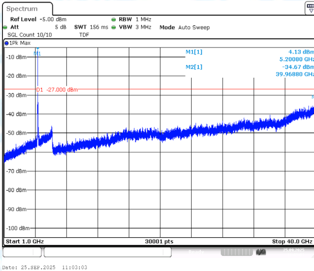
11AC20MIMO-Ant1-5200-1000~40000-PASS
