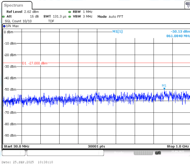
11N40MIMO-Ant1-5190-30~1000-PASS
