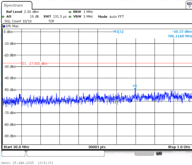
11AC20MIMO-Ant1-5180-30~1000-PASS
