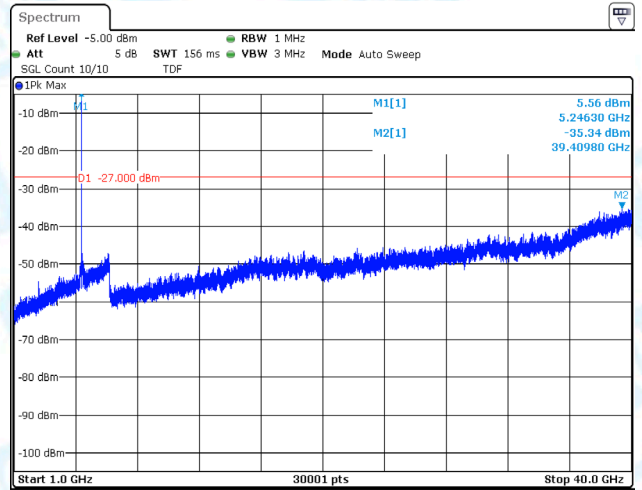
11AC20MIMO-Ant2-5240-1000~40000-PASS
