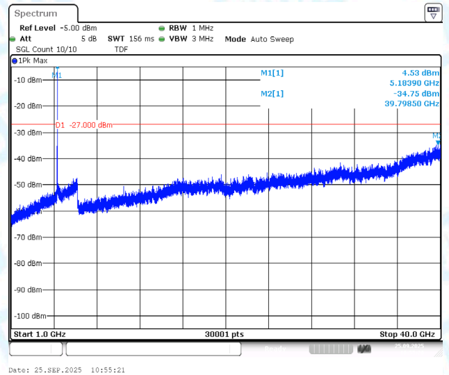
11AC20MIMO-Ant2-5180-1000~40000-PASS
