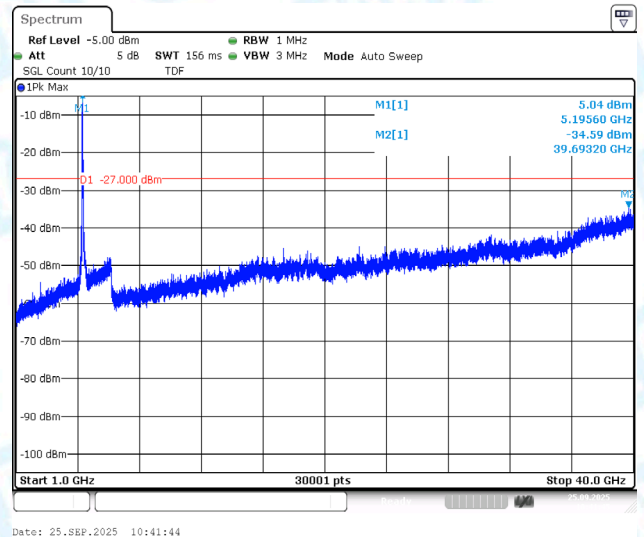
11N40MIMO-Ant2-5190-1000~40000-PASS
