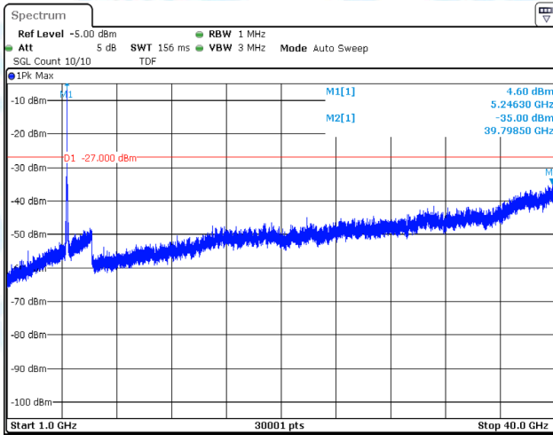
11AC20MIMO-Ant1-5240-1000~40000-PASS
