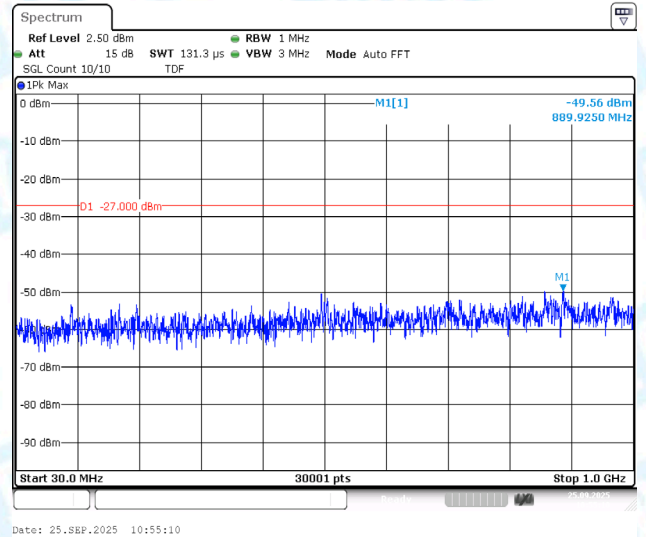
11AC20MIMO-Ant2-5180-30~1000-PASS
