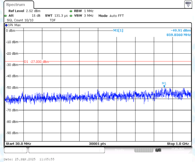
11AC20MIMO-Ant2-5200-30~1000-PASS
