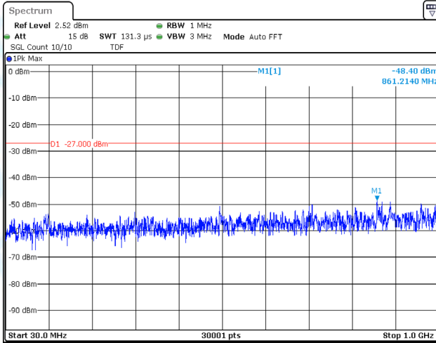
11AC40MIMO-Ant1-5230-30~1000-PASS
