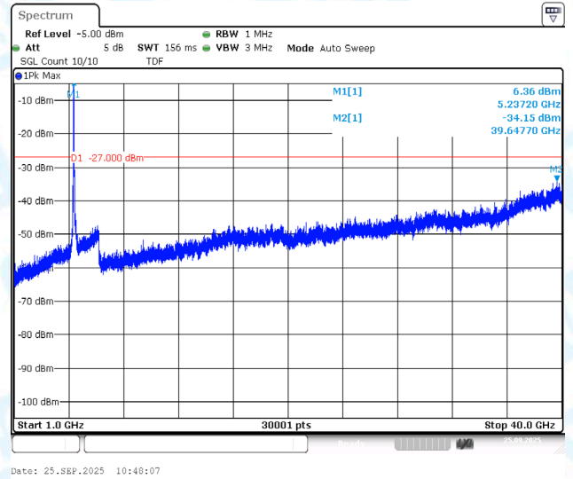
11N40MIMO-Ant2-5230-1000~40000-PASS
