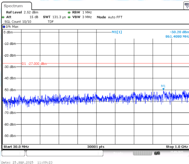
11AC20MIMO-Ant1-5240-30~1000-PASS
