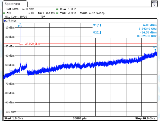
11AX20MIMO-Ant2-5240-1000~40000-PASS
