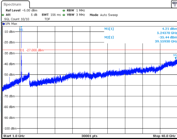
11AX20MIMO-Ant1-5240-1000~40000-PASS
