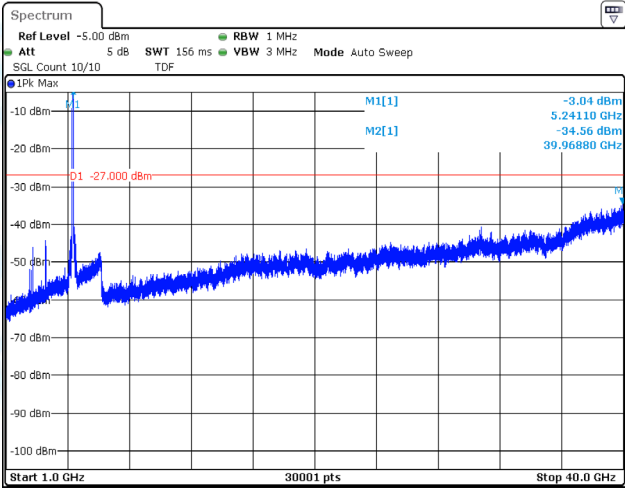
11AX80MIMO-Ant1-5210-1000~40000-PASS
