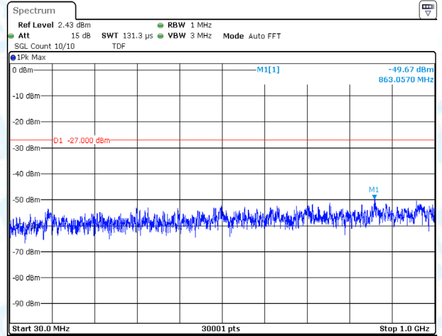
11AX40MIMO-Ant2-5230-30~1000-PASS
