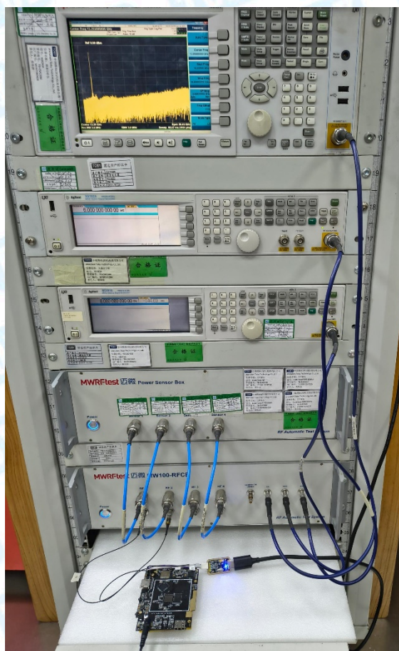
Photo of Setup for Conducted Measurement
