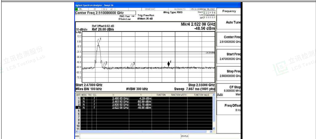
BLE_2M_Ant1_High_2480
