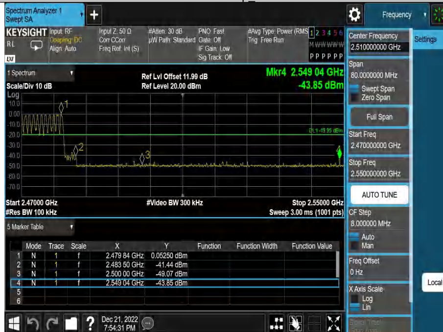
DH5-Ant1-High-Hop_2480-0.05
