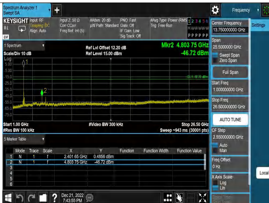
DH5-Ant1-2402-1000~26500-1.30
