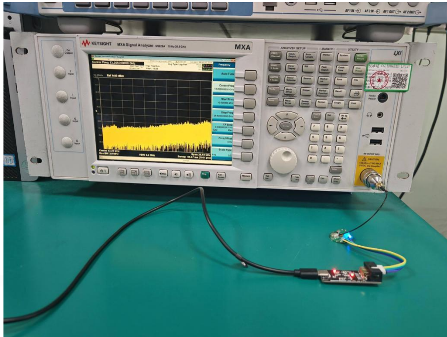
RF Conducted
