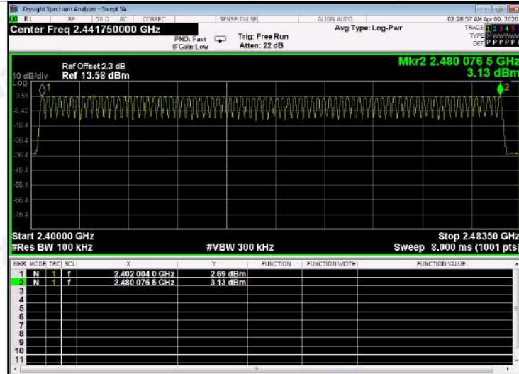
GFSK Modulation
