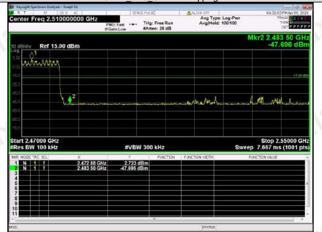
Out Of Band Emission(Right) π/4DQPSK 2-DH5 Channel Hopping
