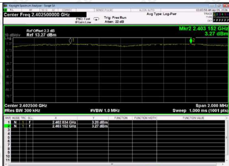
8-DPSK
