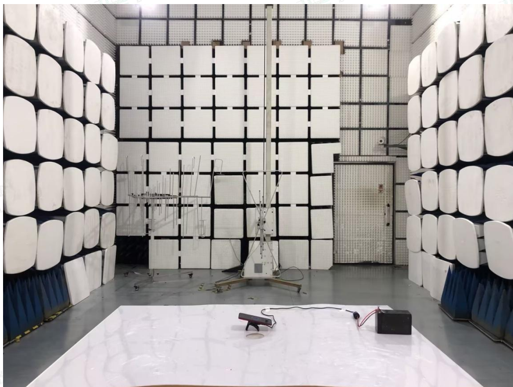
Radiated Emission below 1GHz-TM1
