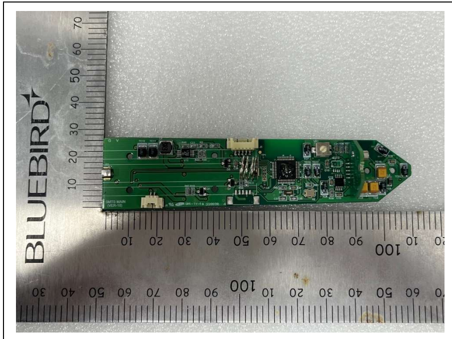
Main board_Bottom
