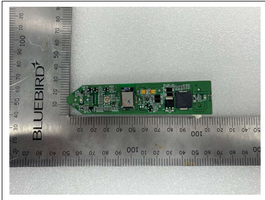
Main board_Top
