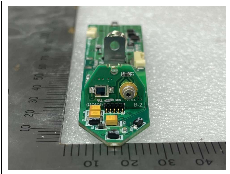
Sub board_Top
