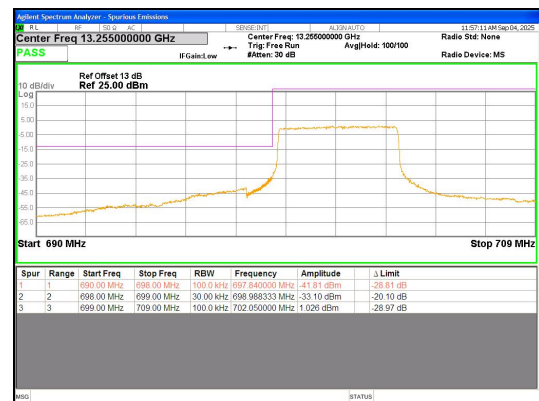
Band 12 5MHz/701.5/Low 16QAM 1@0
