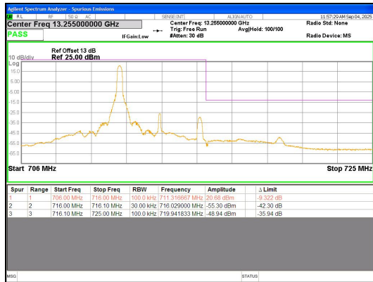
Band 12 5MHz/713.5/High QPSK 1@0
