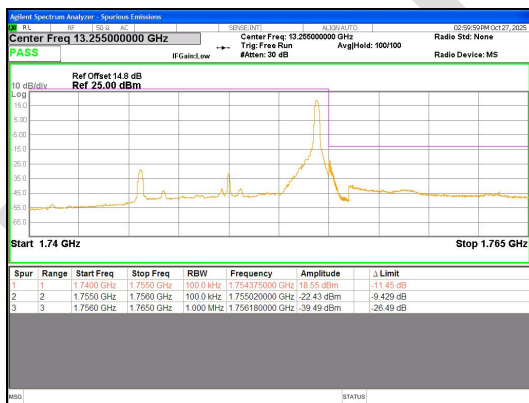
Band 4 10MHz/1750.0/High QPSK 50@0
