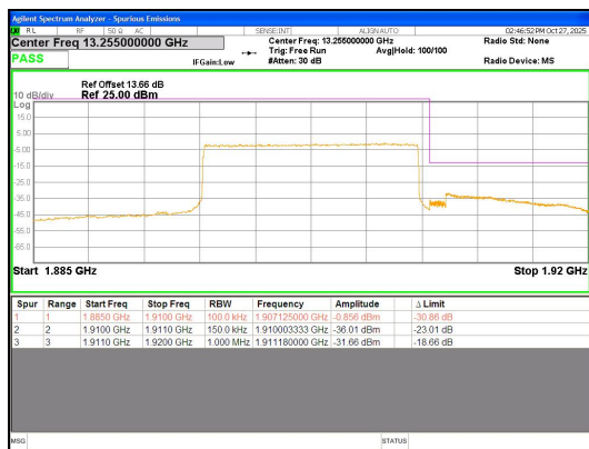
Band 2 15MHz/1902.5/High QPSK 1@0
