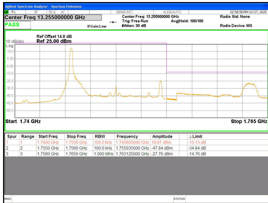
Band 4 10MHz/1750.0/High QPSK 1@0
